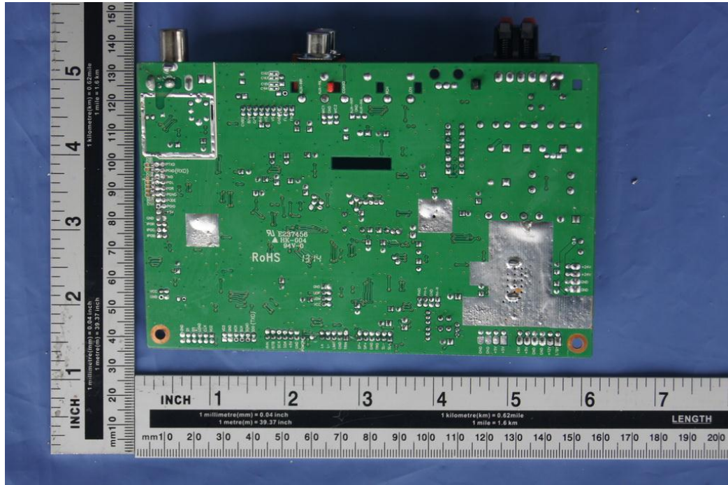
Fig. 7: Internal view
