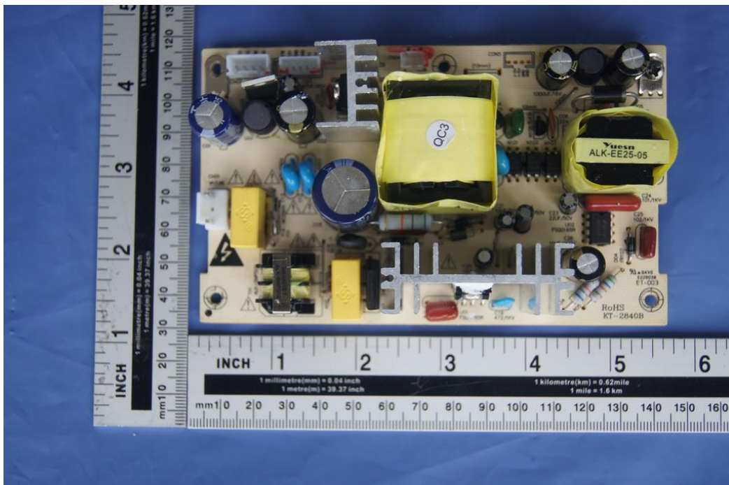
Fig. 2: Internal view
