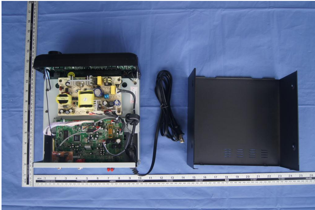
Fig. 1: Internal view
