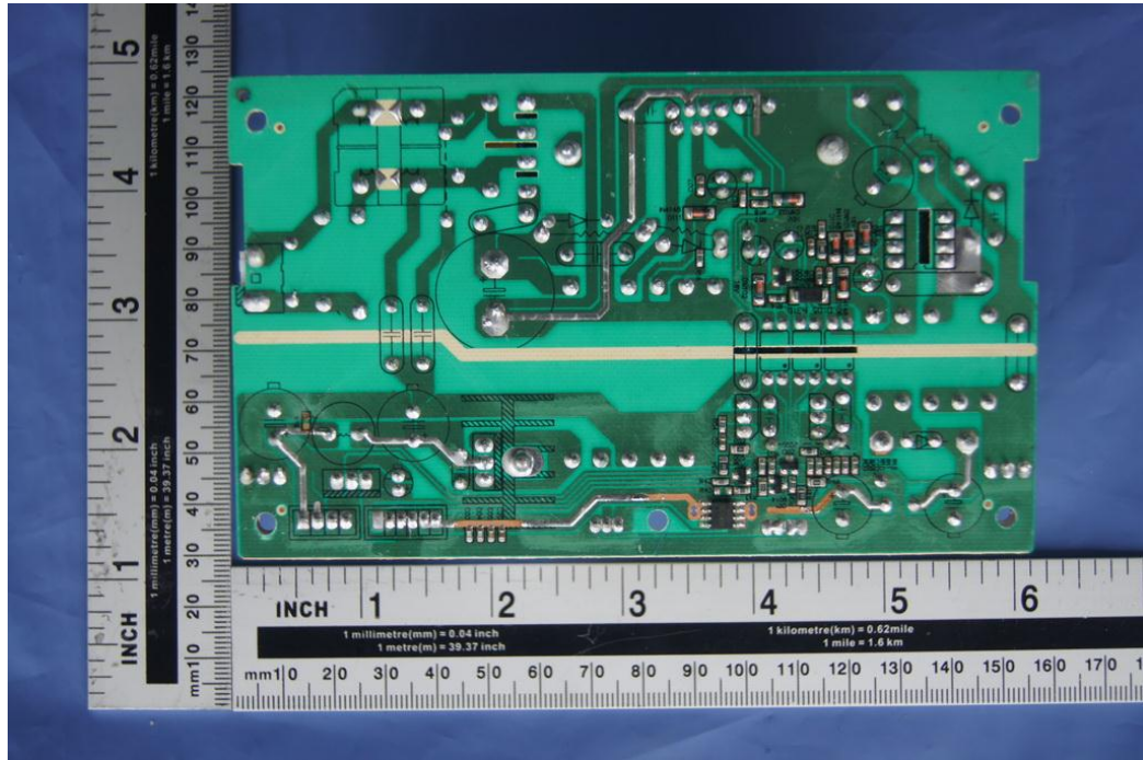
Fig. 3: Internal view
