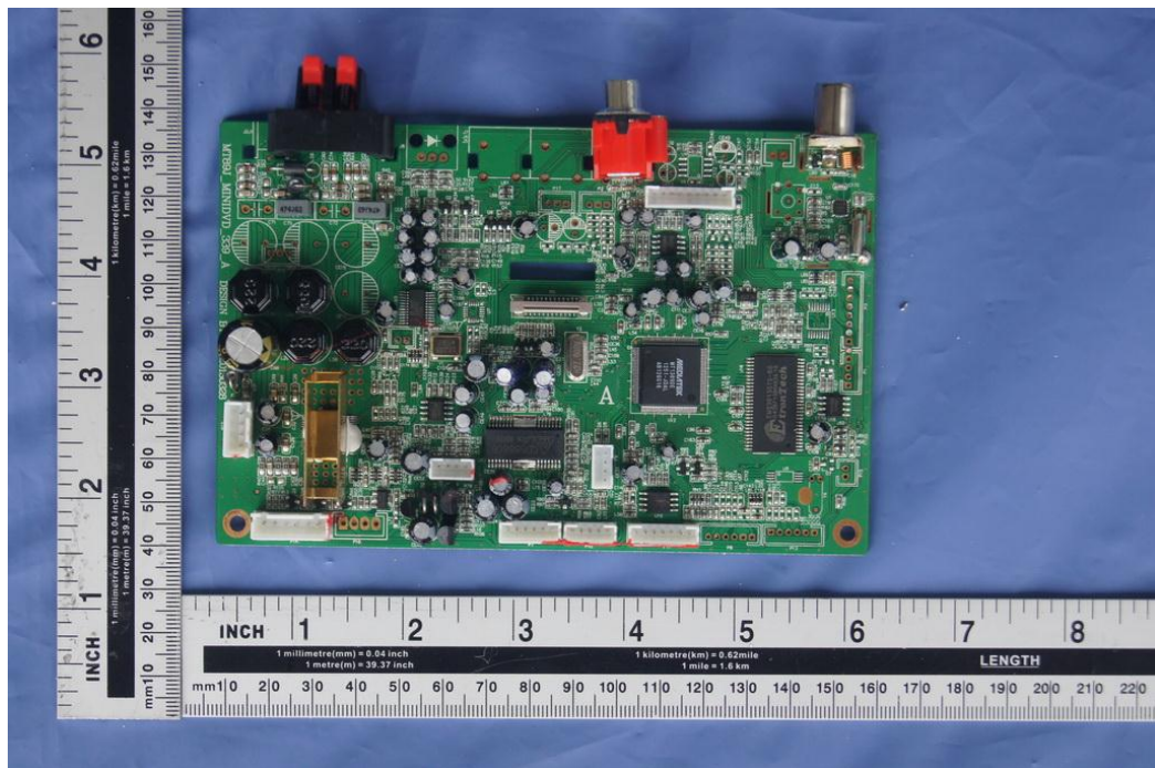
Fig. 6: Internal view
