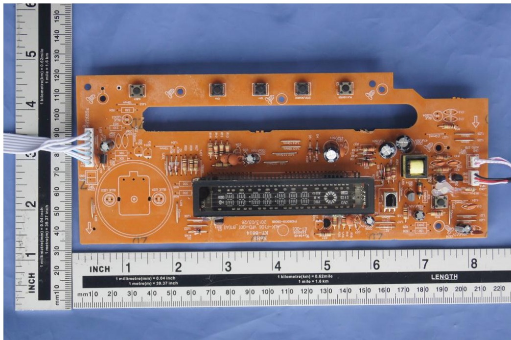
Fig. 4: Internal view
