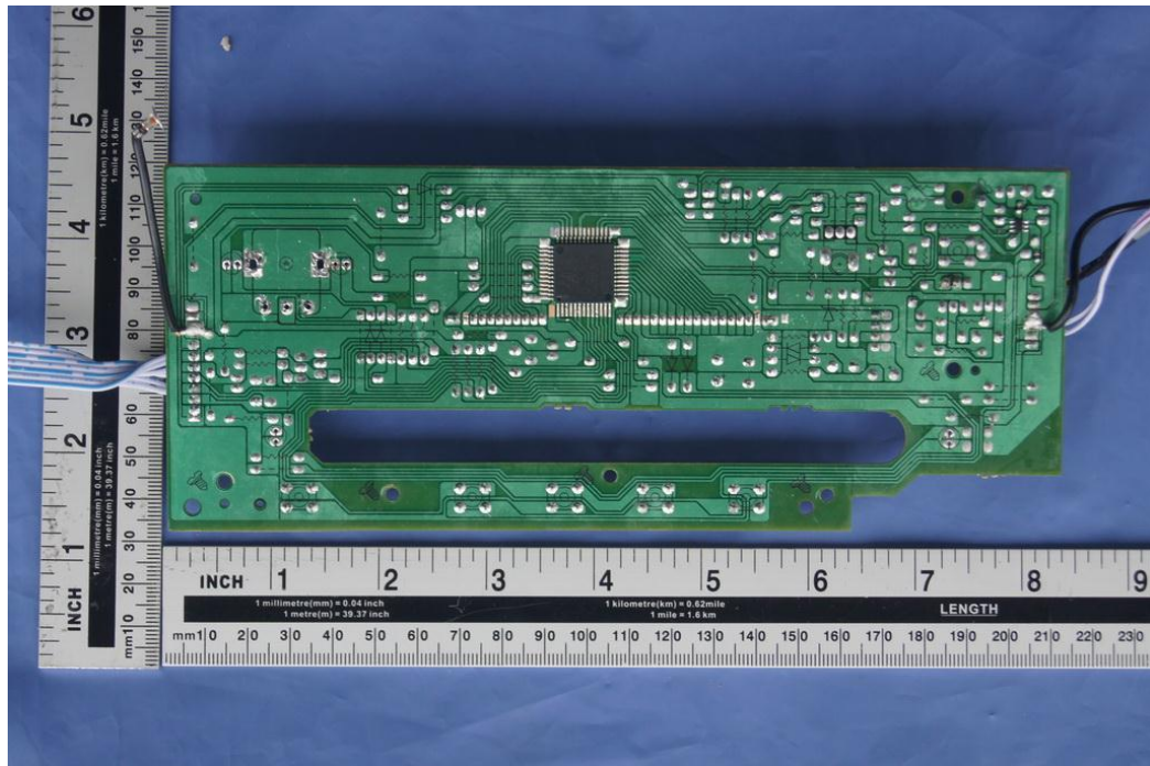
Fig. 5: Internal view
