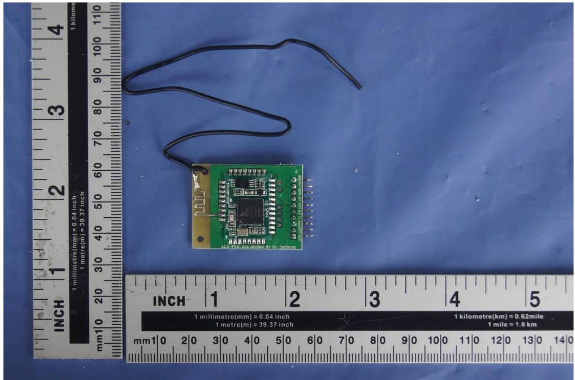
Fig. 9: Internal view
