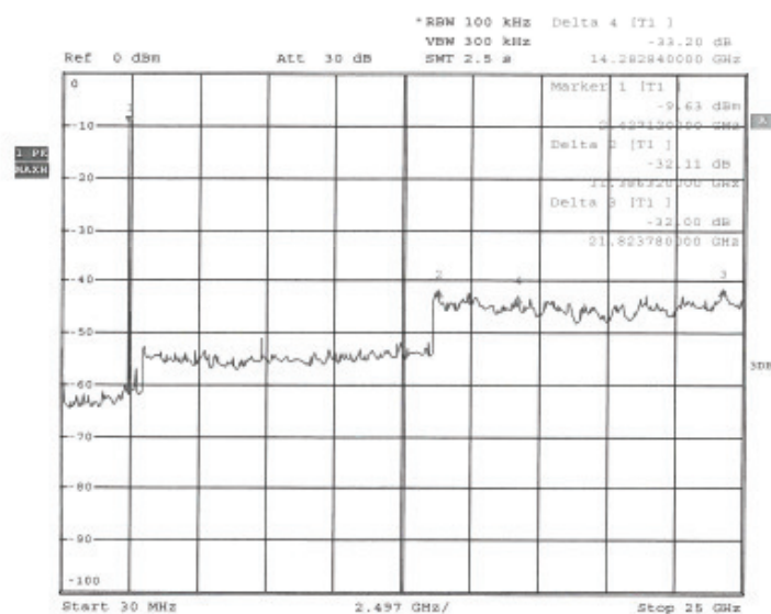
20140828 ITS8-300W Conducted Spurious Emission M (BR)
