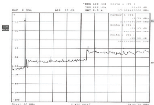
20140828 ITSB-300W Conducted Spurious Emission L (BR)
