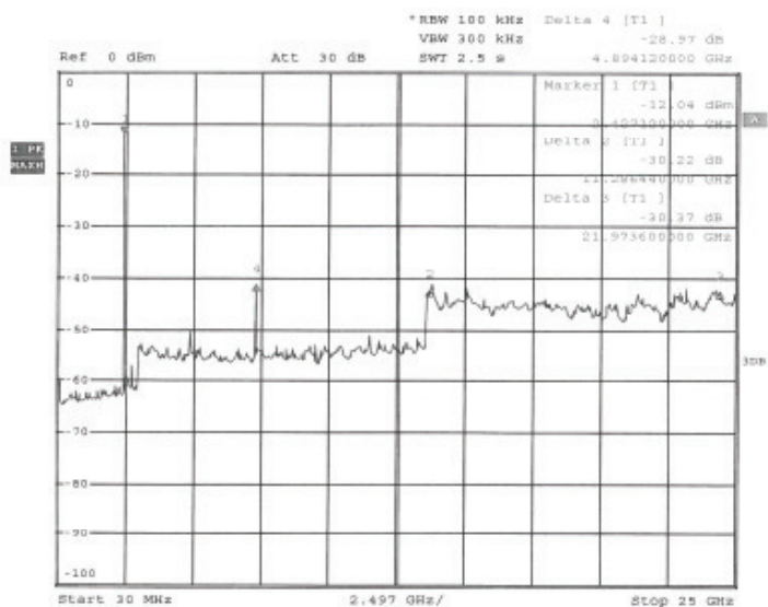
20140828 ITS8-300W Conducted Spurious Emission M (EDR)
