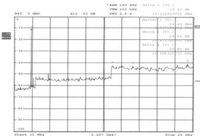
20140828 ITSB-300W Conducted Spurious Emission L (EDR)
