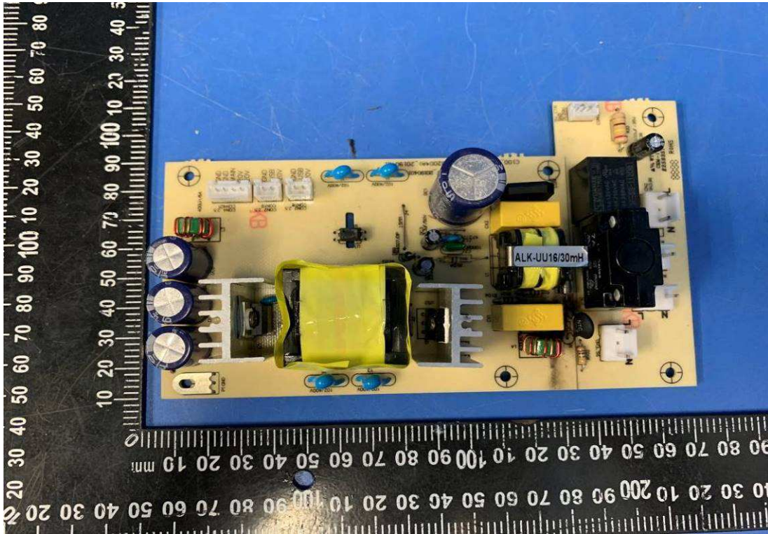
Picture 5. Power board 1
