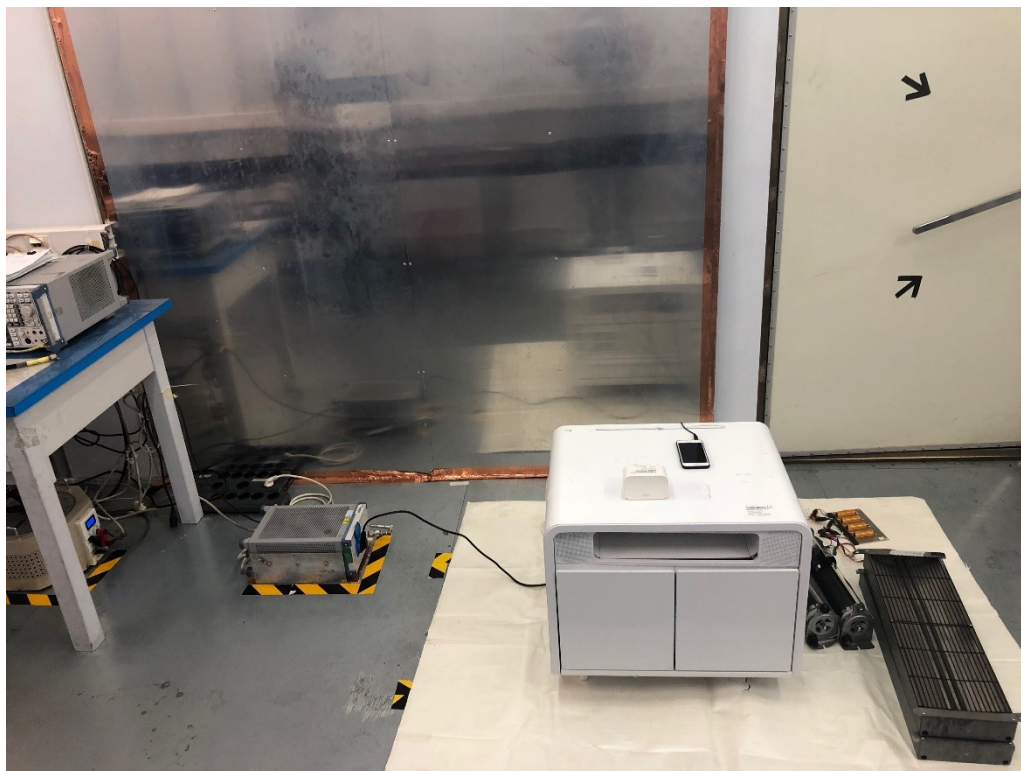
Photograph 5: Set-up for Conducted Emission on AC Mains
