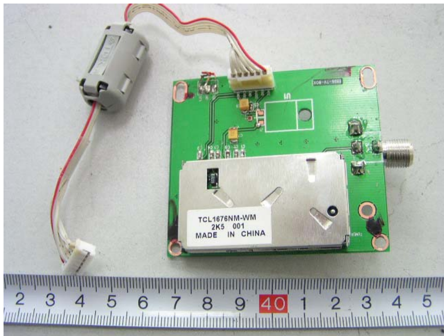
EUT –TV Tuner-1 View
