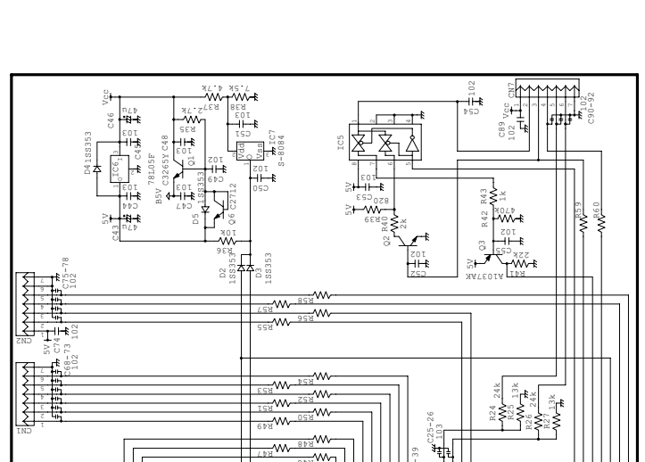
FCC ID# BRWX378 Figure 5.2.1. Transmitter Schematic Diagram
