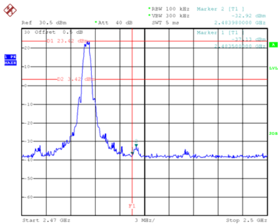
GFSK Transmitting Band edge-right side
