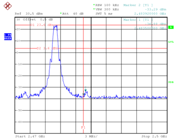
2.4G(ANT 2): Band edge-right side
