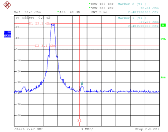
2.4G(ANT 1): Band edge-right side
