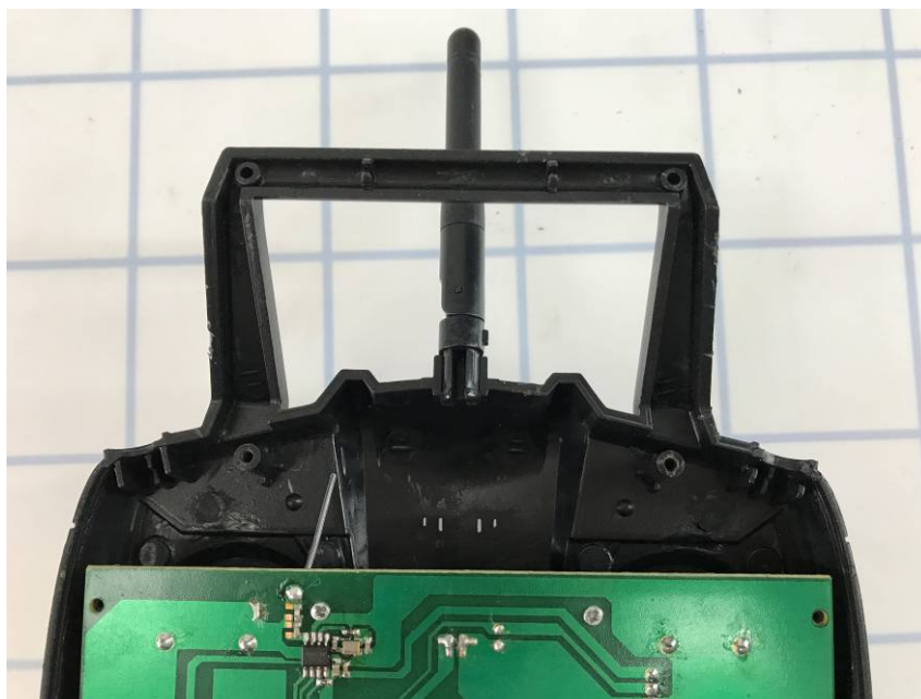
Antenna close up photo view 2
