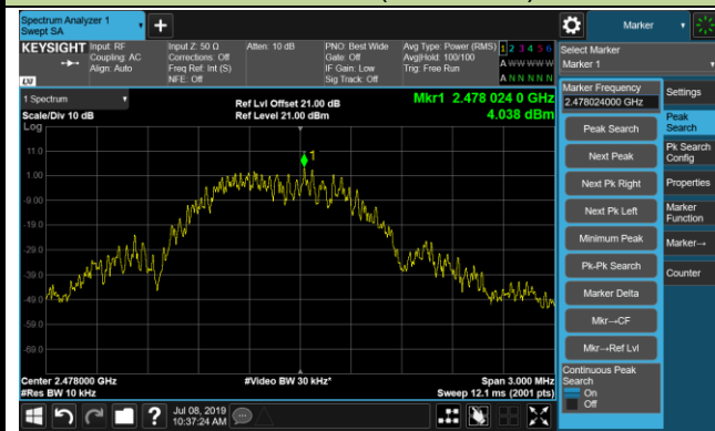
Channel 23 (2478MHz)
