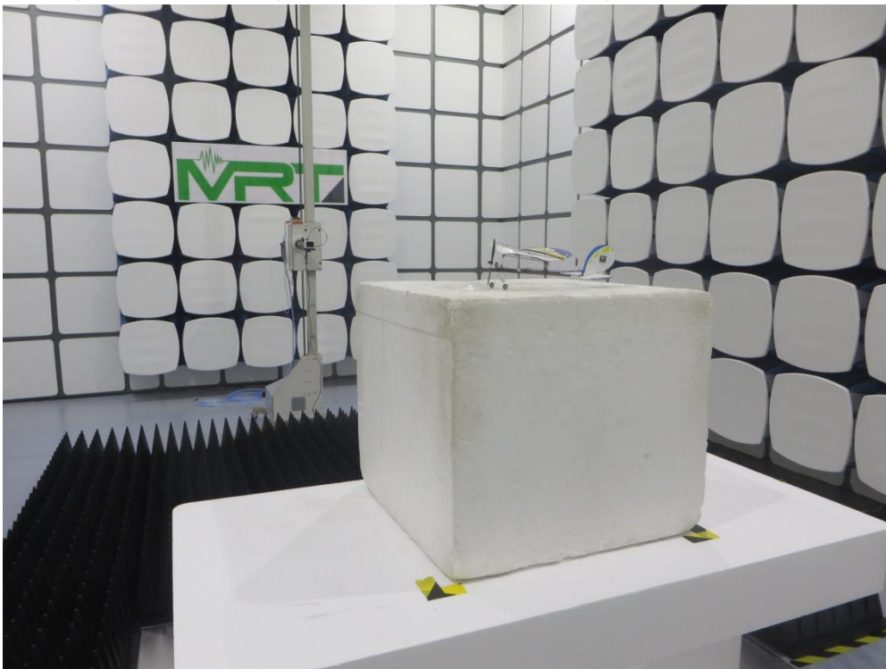
Description: Radiated Spurious Emissions Test Setup for 18 ~ 25GHz
