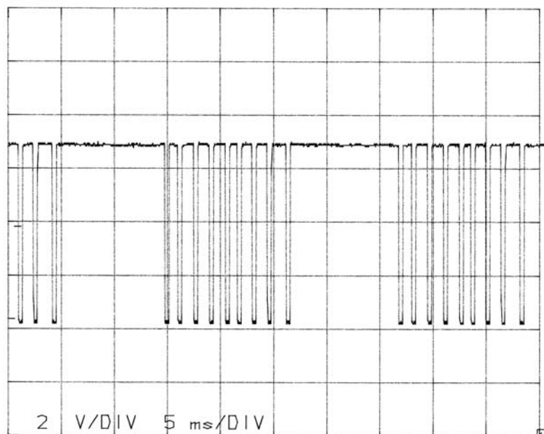
Encoded Waveform (PPM Modulation)
