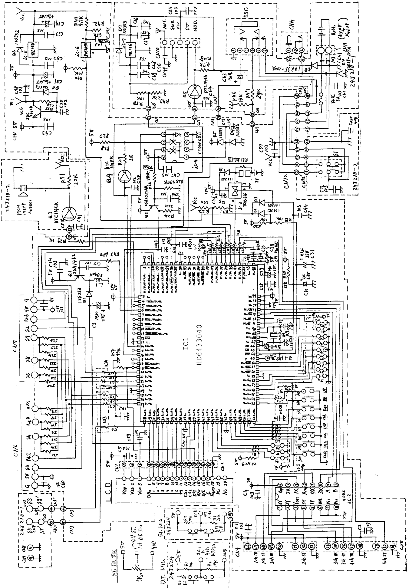
FCC ID# BRWNETJS725SYN Figure 5.2.2 Transmitter Schematic Diagram
