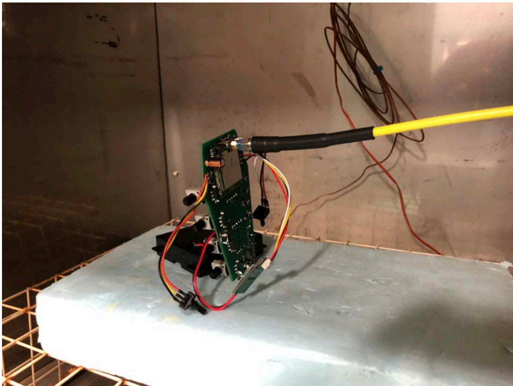
Test Setup for Antenna Conducted Tests
