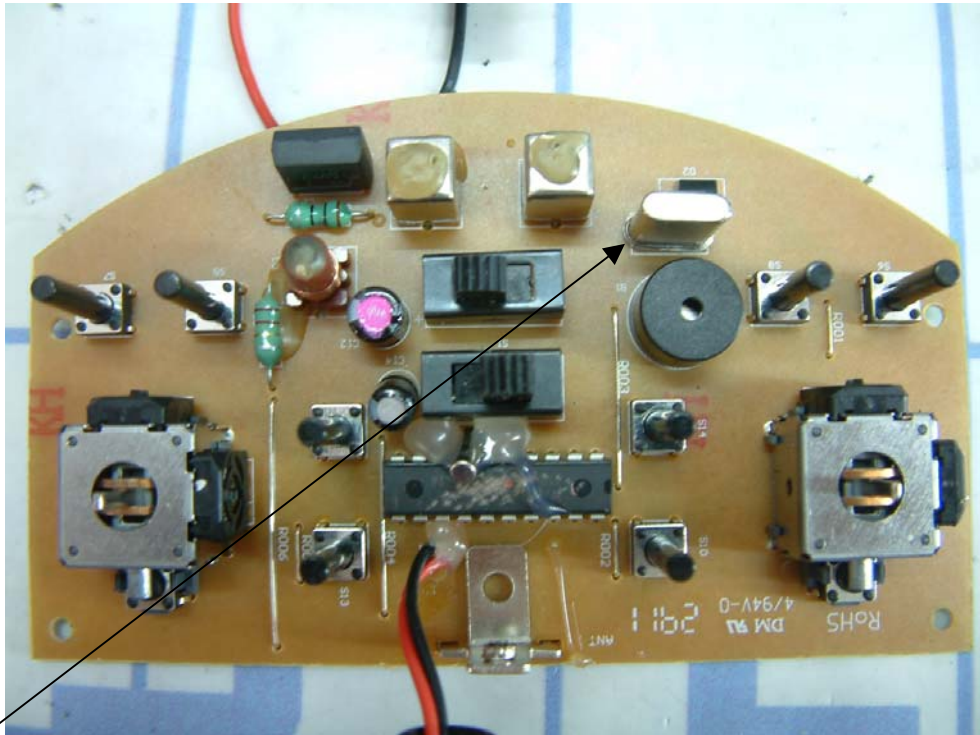
HBZ 4776 PCB Layout view-2
