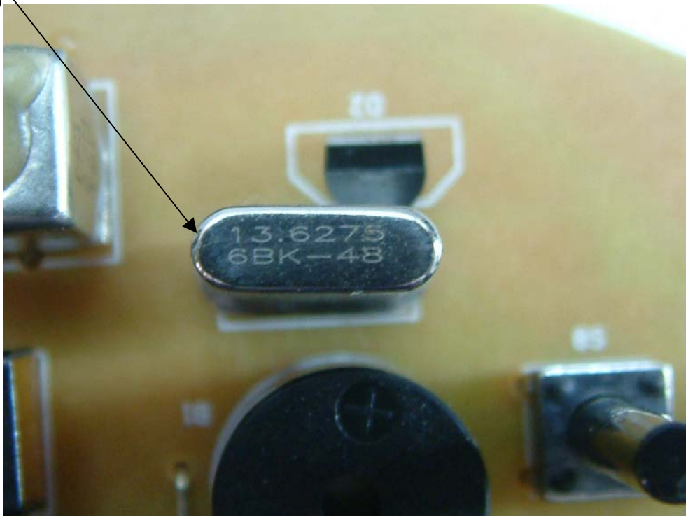
HBZ 4776 Crystal location
