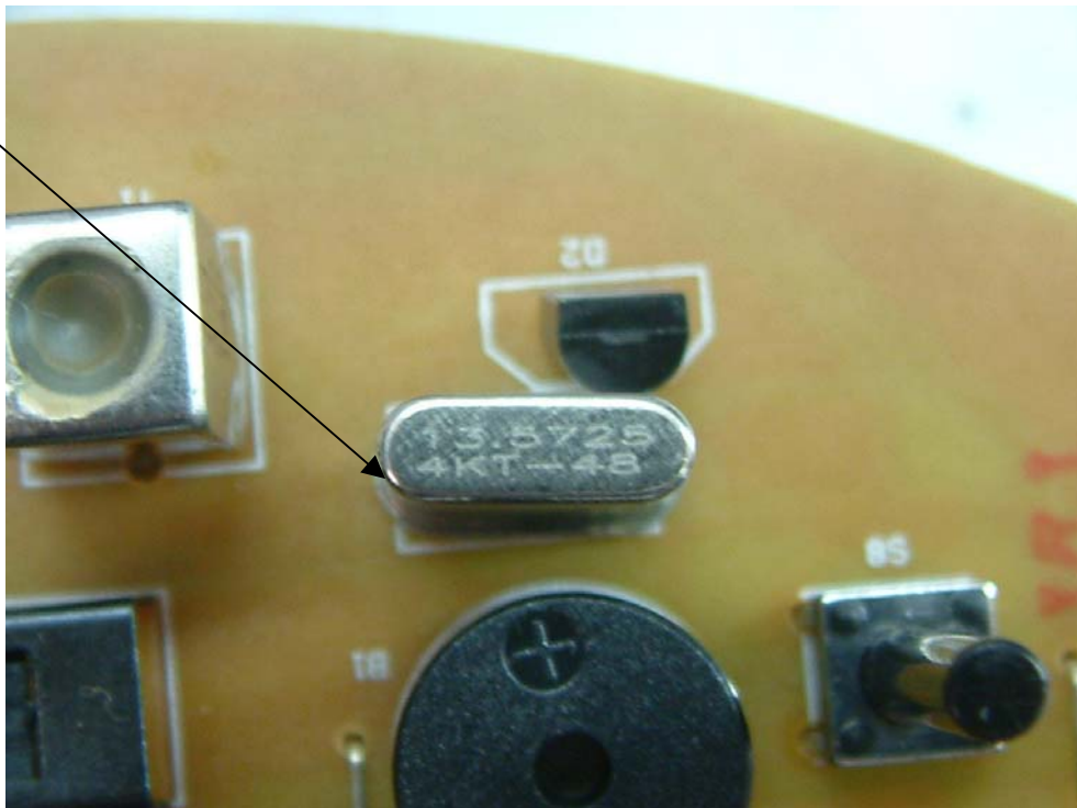
HBZ 4771 Crystal location
