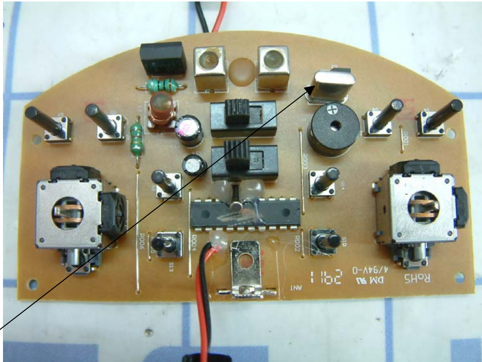
HBZ 4774 PCB Layout view-2
