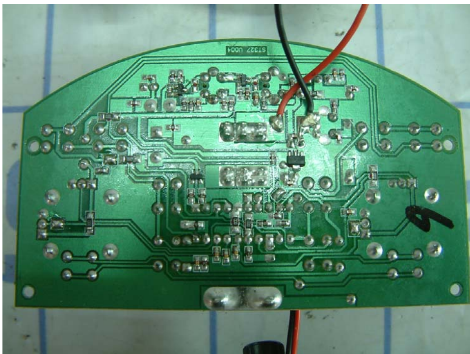
HBZ 4776 PCB Layout view-1
