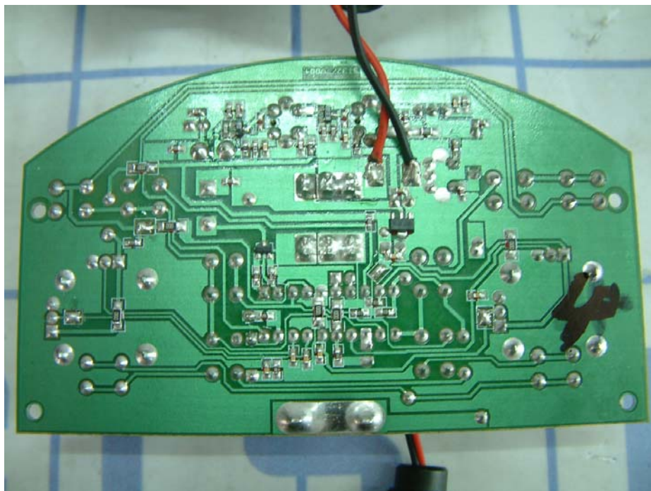
HBZ 4774 PCB Layout view-1
