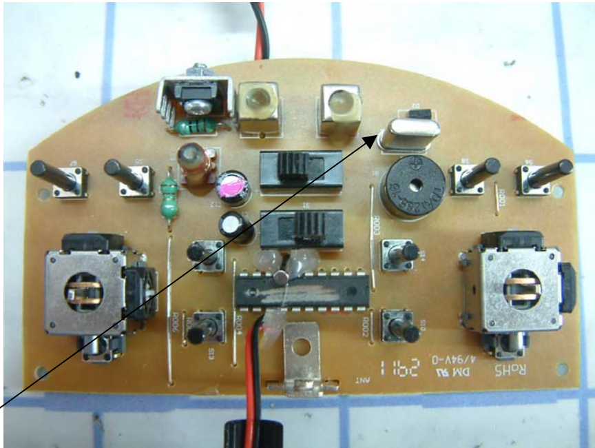
HBZ 4771 PCB Layout view-2
