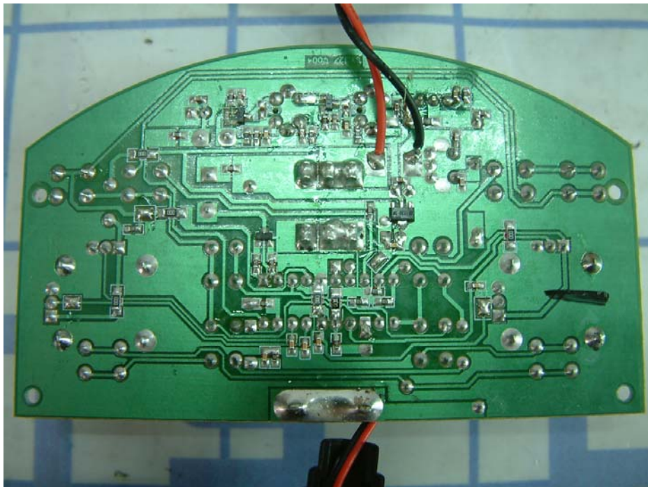
HBZ 4771 PCB Layout view-1
