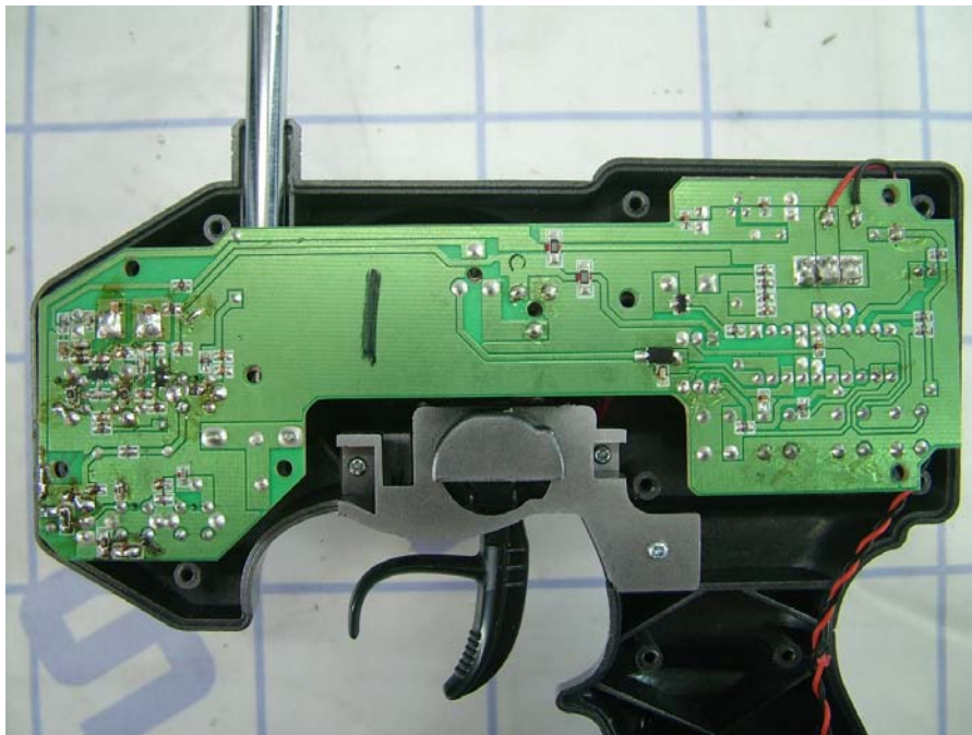
HBZ3751 PCB Layout view-1
