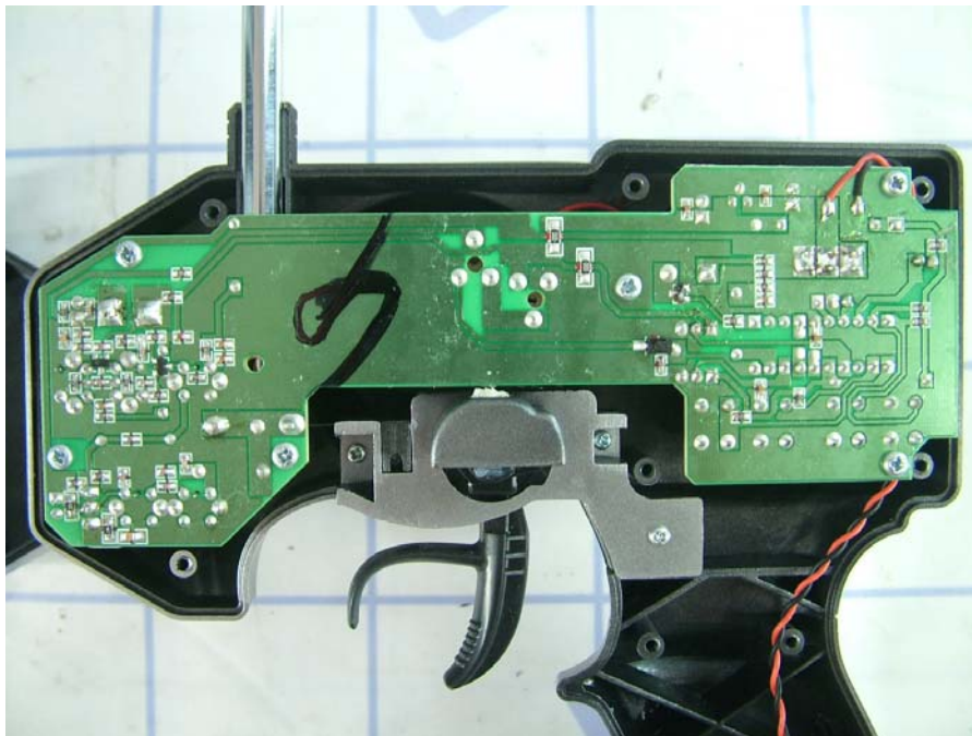
HBZ3754 PCB Layout view-1
