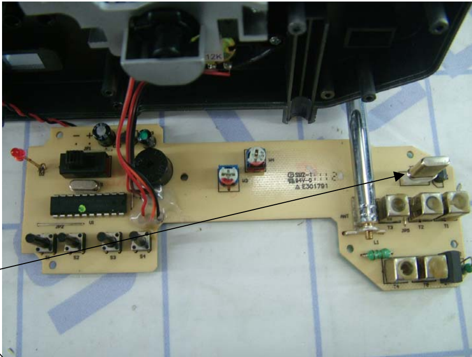
HBZ3756 PCB Layout view-2
