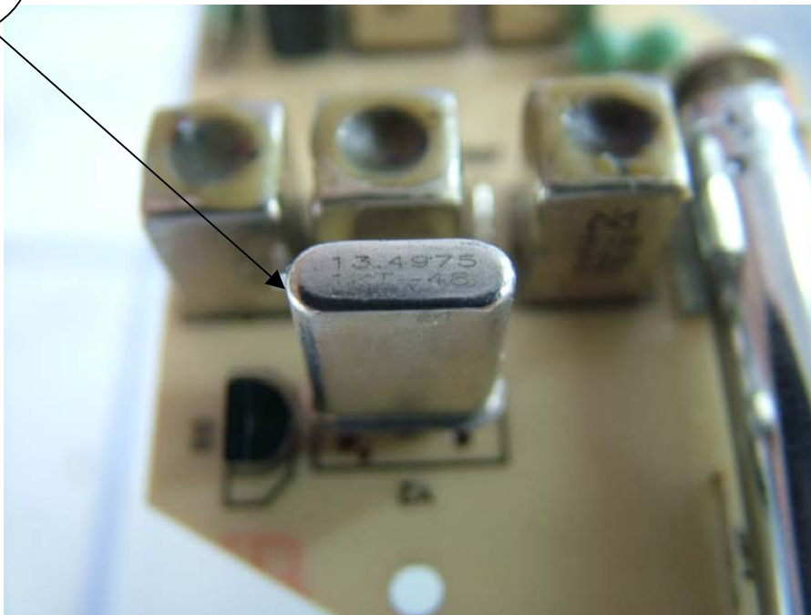
HBZ3751 Crystal location
