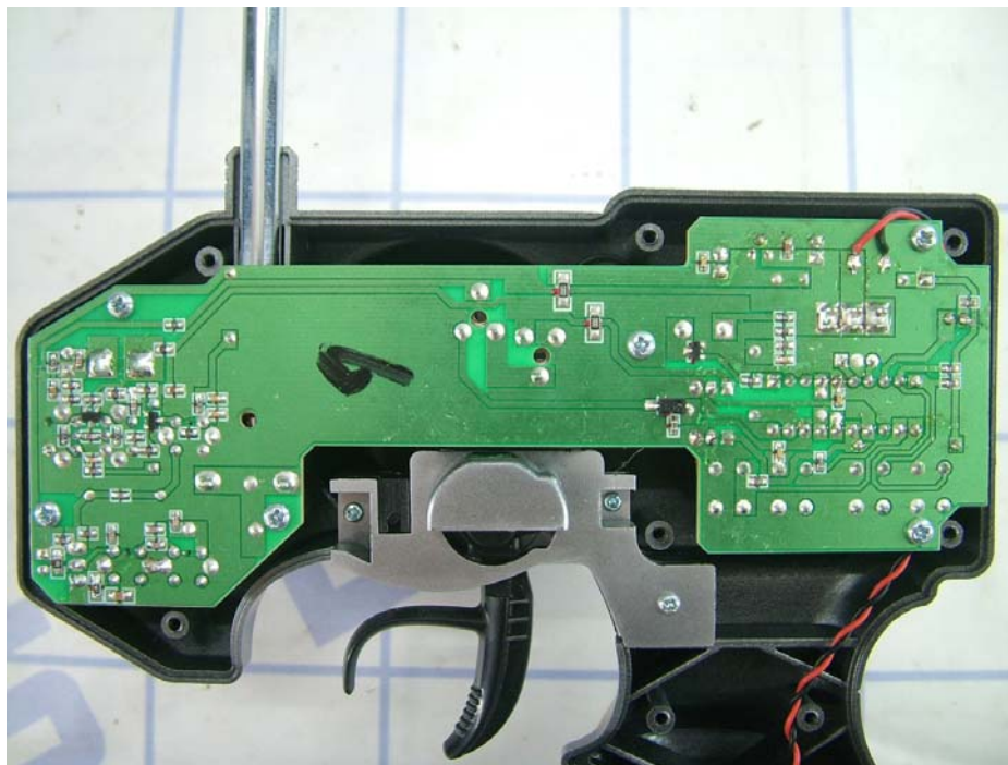
HBZ3756 PCB Layout view-1
