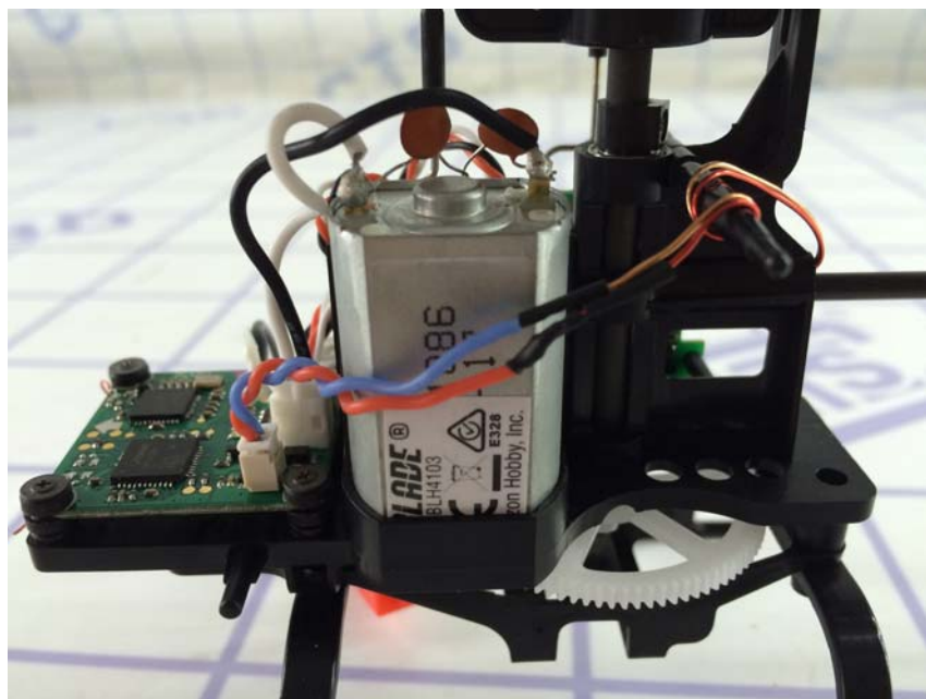
Motor view
