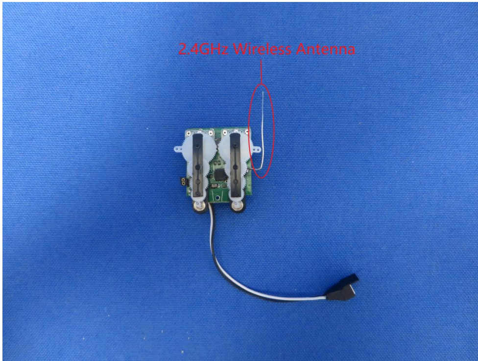
(1) EUT Photo
