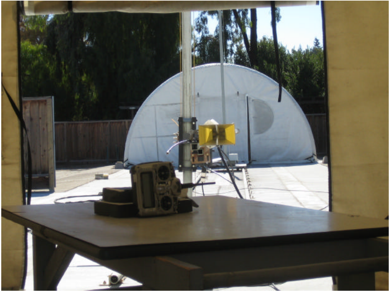
Test fixture on its side for radiated emissions measurements
