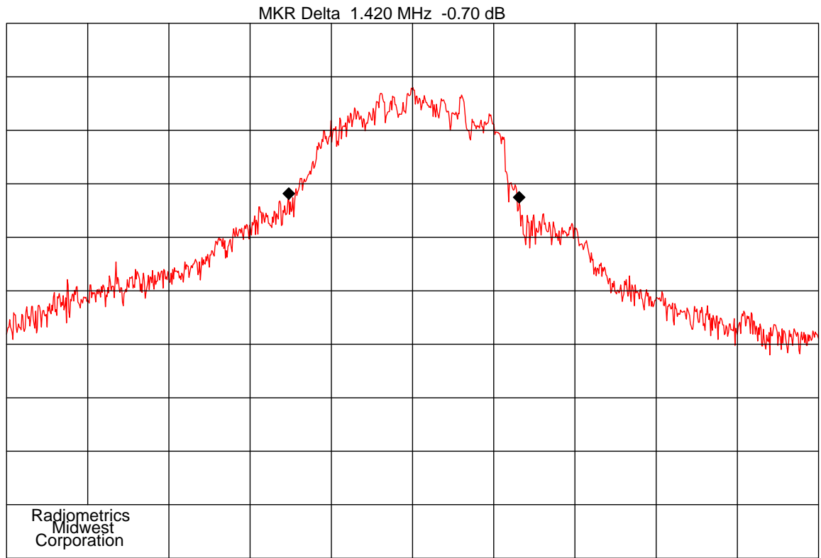
Figure 2. Occupied Bandwidth Plots
