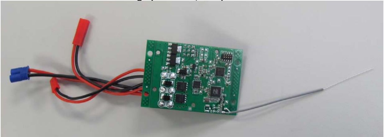
Photograph of PCB; Component Side
