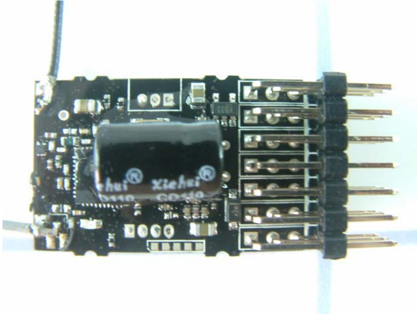
PCB view -1
