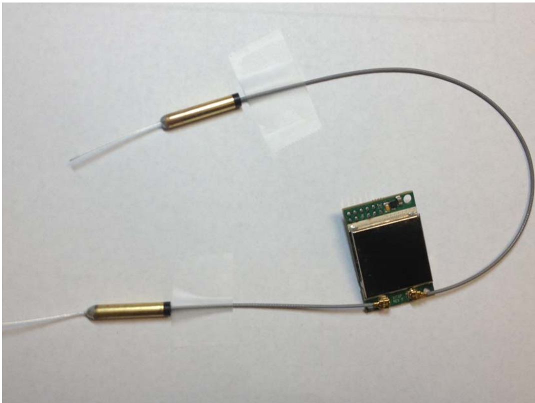
Bottom of EUT: antenna attached
