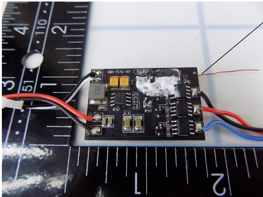
PCB side 2
