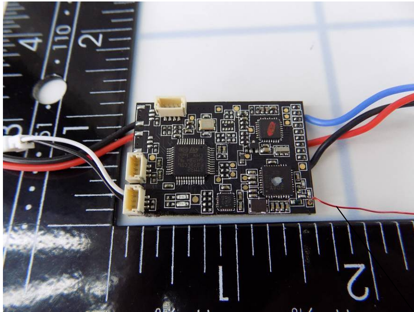
PCB side 1
