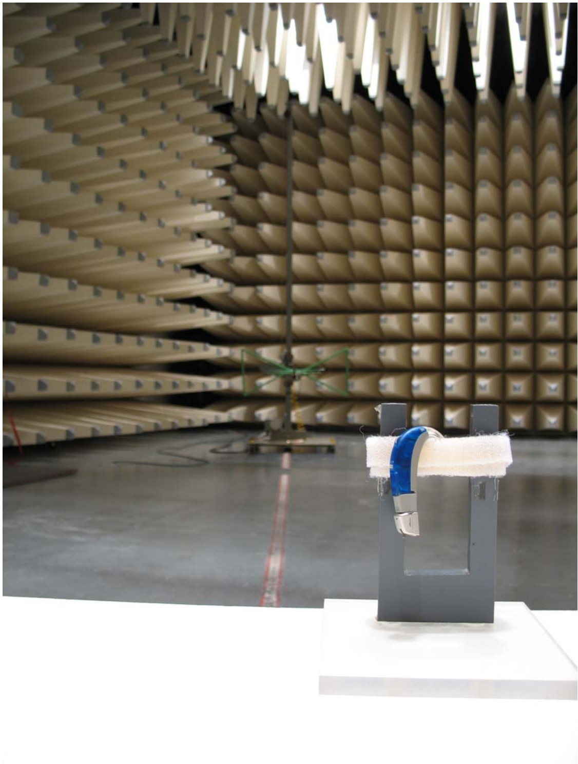
Photo 1 (Radiated Emissions):
