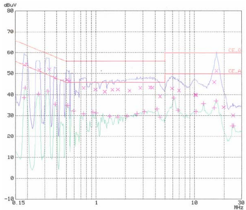
< Neutral line >
