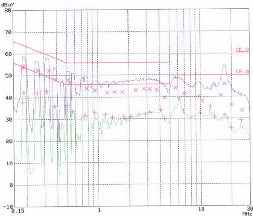
< Hot line >
