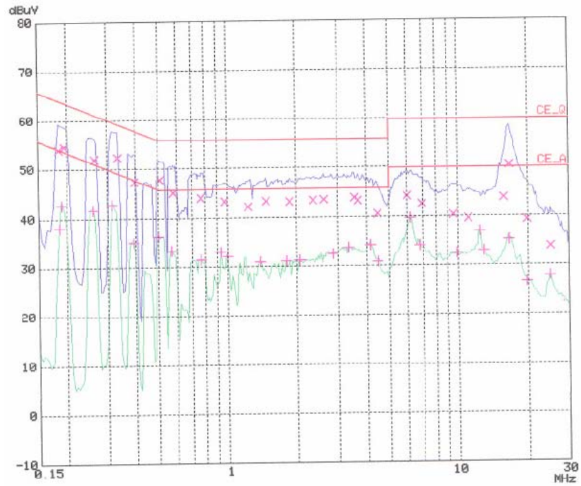
< Hot line >
