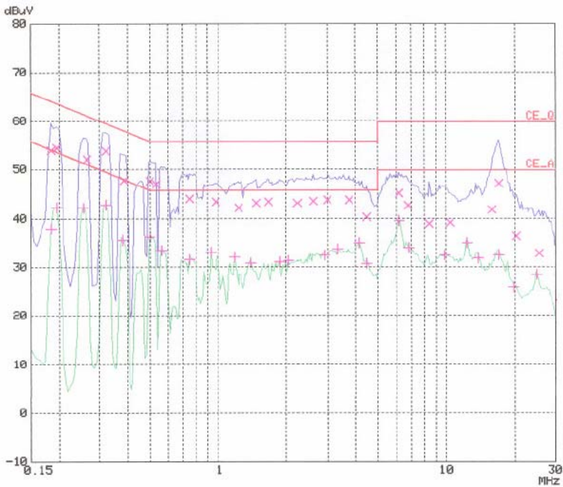
< Hot line >
