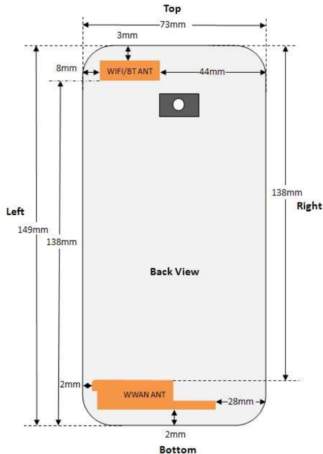
Fig.14.1 EUT Antenna Locations
