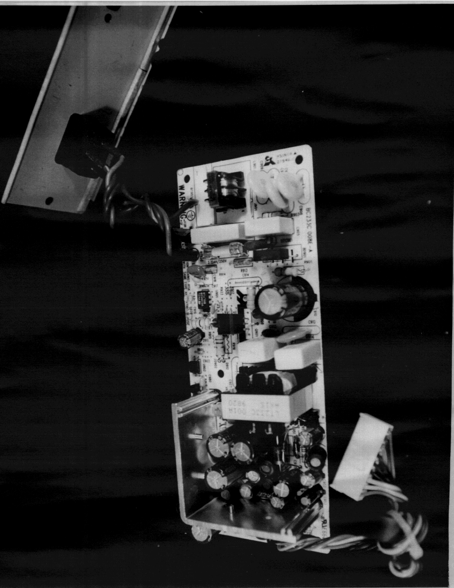
FCC ID. : BR8DV-821 E.U.T. : DIGITAL SATELLITE RECEIVER Component View of Power PCB
