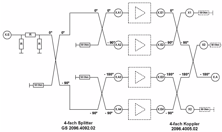
Fig. 20 Block diagram of the output stage unit - in this example NW8204
