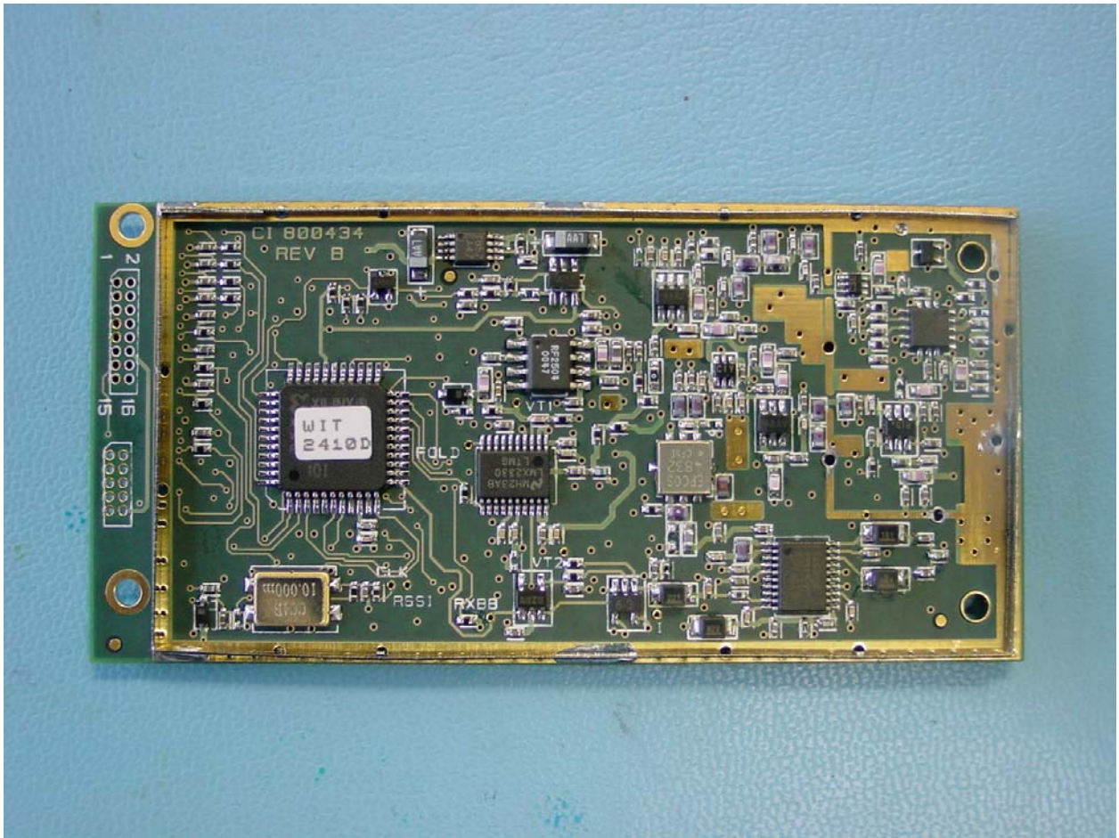
Photo 7. EUT, Top View of Transceiver Board
