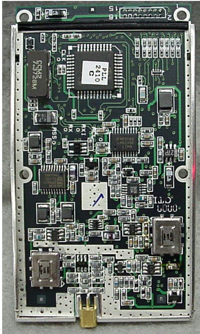
Photo 9. EUT, Top View of Transceiver Board
