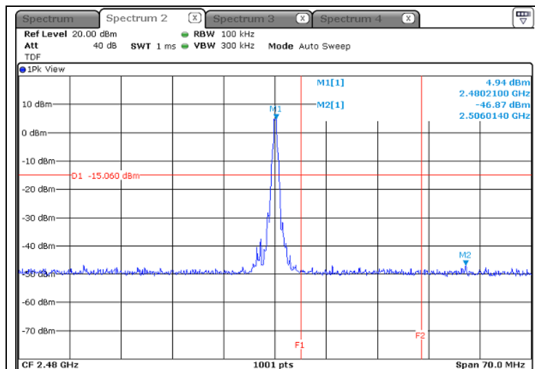
- Result of 2 483.5 MHz (F1:2 483.5 MHz, F2: 2 500 MHz)
