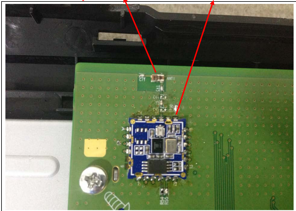
Chip Antenna & Bluetooth Module
