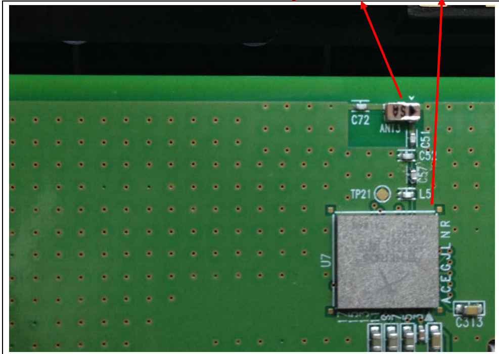
Chip Antenna & WIFI Module
