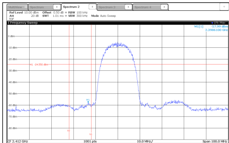
- Result of 2 400.0 MHz (F1:2 390 MHz, F2:2 400 MHz)
