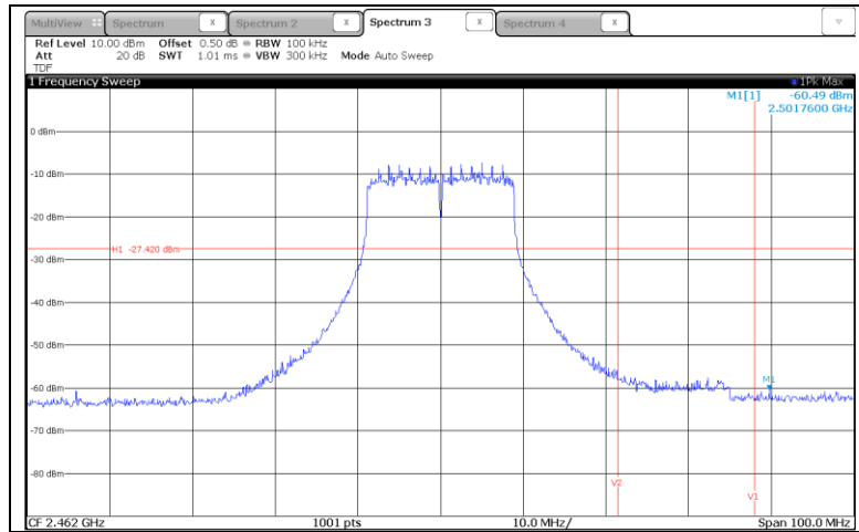
- Result of 2 483.5 MHz (F1:2 483.5 MHz, F2:2 500 MHz)
