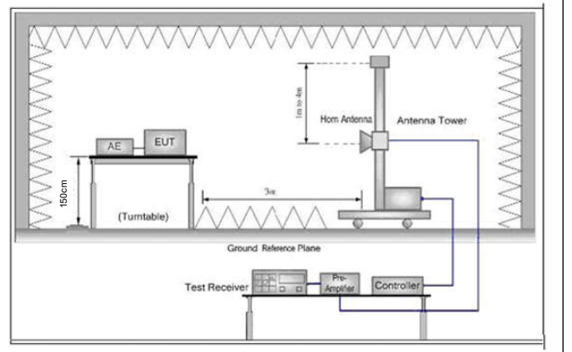
Figure 3. Above 1 GHz
