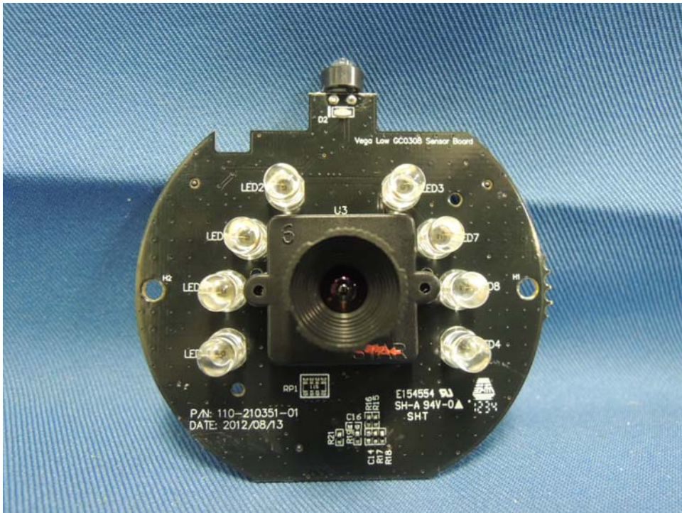
Baby Unit Cam & LED Board front side
