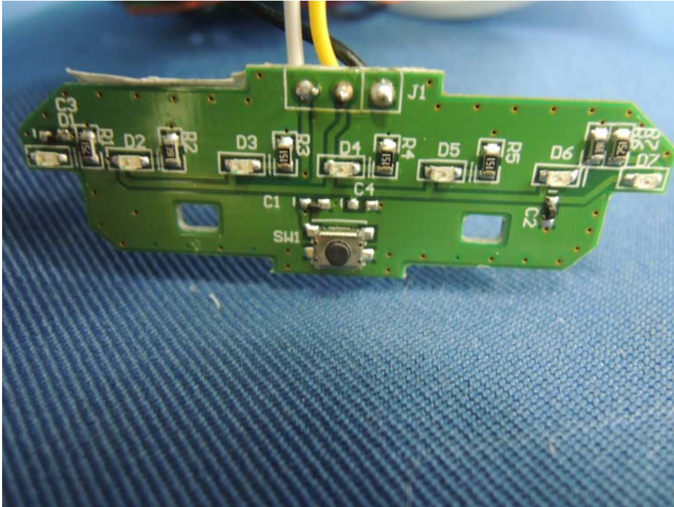
Baby Unit LED Power Board rear side
