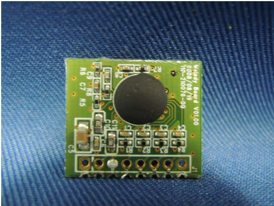
Baby Unit Melody Board front side
