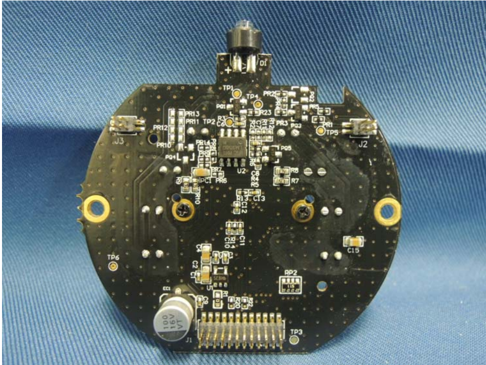
Baby Unit Cam & LED Board rear side
