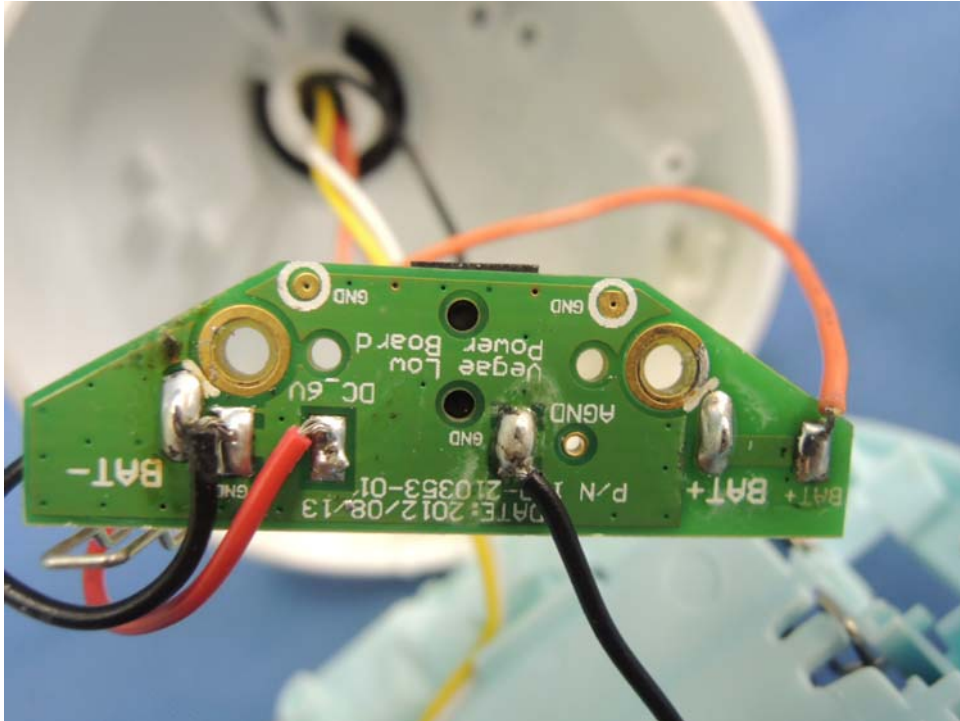
Baby Unit Power Board rear side
