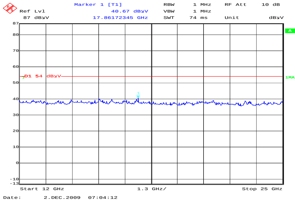
Plot 3: 12 - 25 GHz, antenna vertical/horizontal (receiver)
