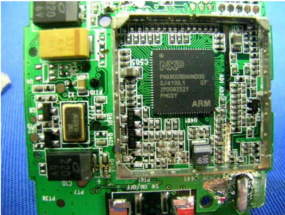
Parent Unit DECT RF Module comp side
