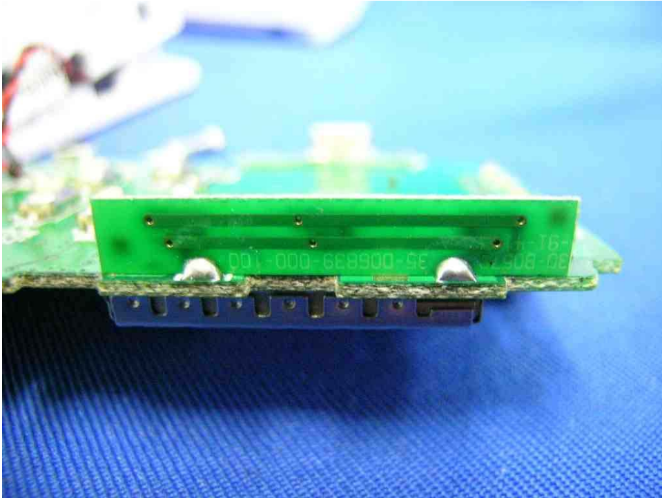
Parent Unit Main PCB solder side (View 4)
