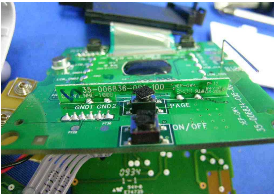
Baby Unit Main PCB solder side (View 5)
