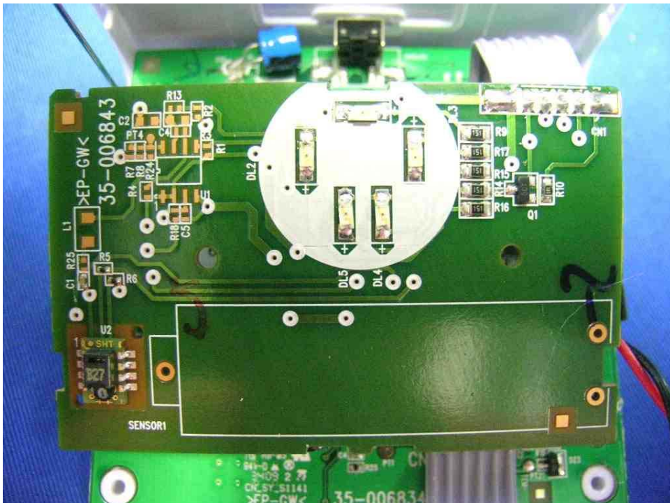
Baby Unit Night Light PCB front side
