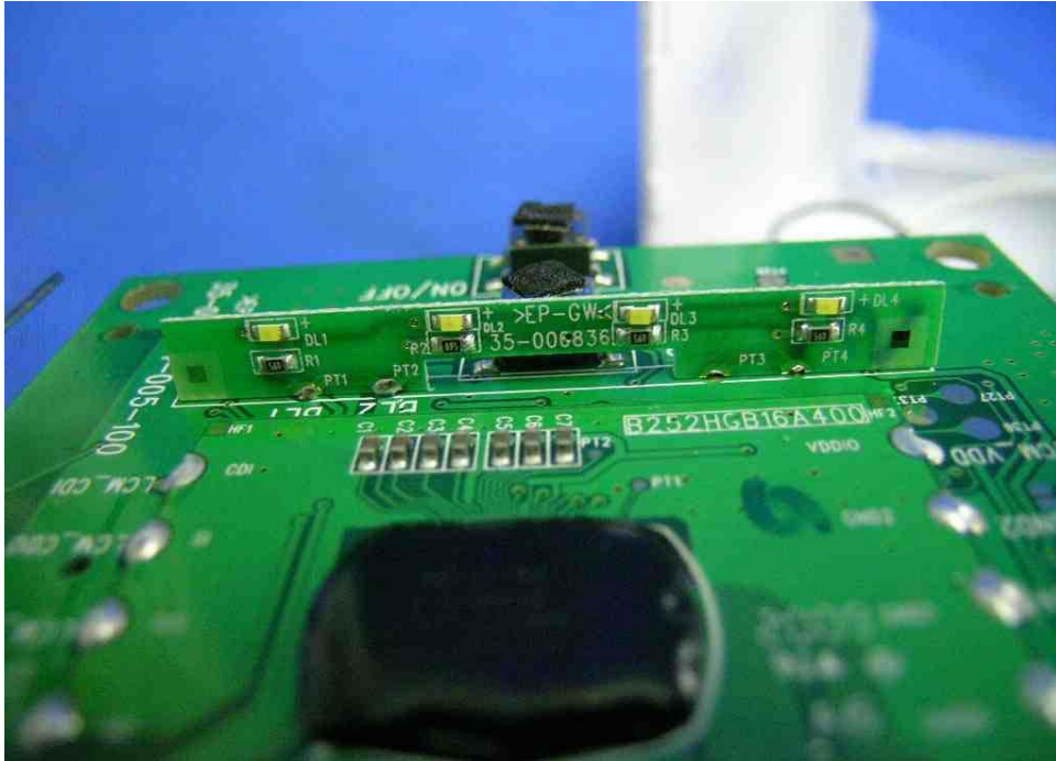
Baby Unit Main PCB solder side (View 4)
