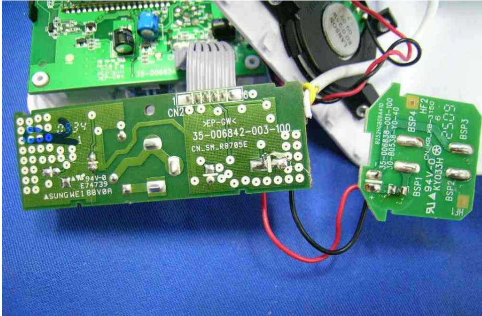
Baby Unit Power Supply PCB & Battery Contact PCB rear side
