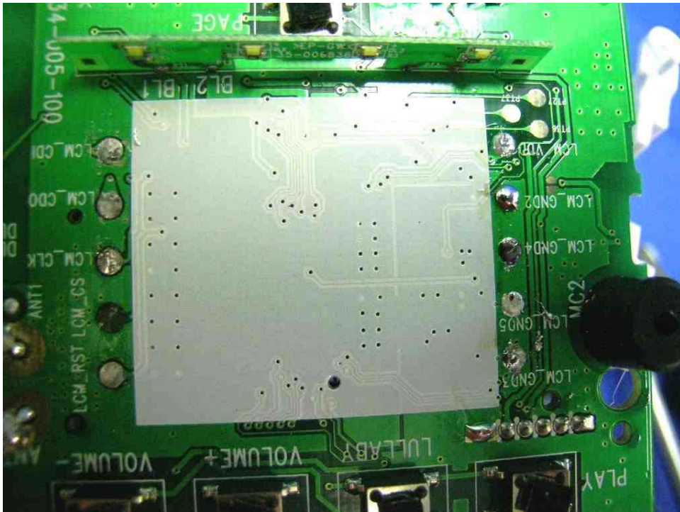
Baby Unit Main PCB solder side (View 3)
