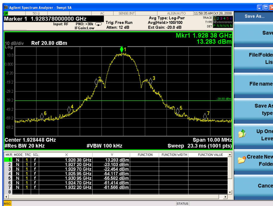
Upper Channel
