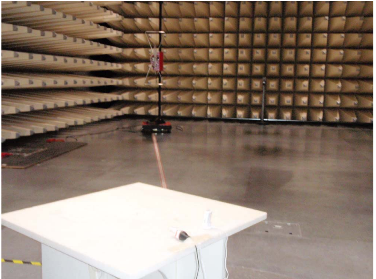
Photo 2: Radiated Emission and Antenna Gain Test
