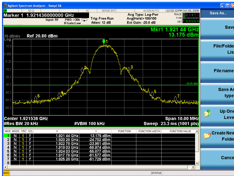
Lower Channel
