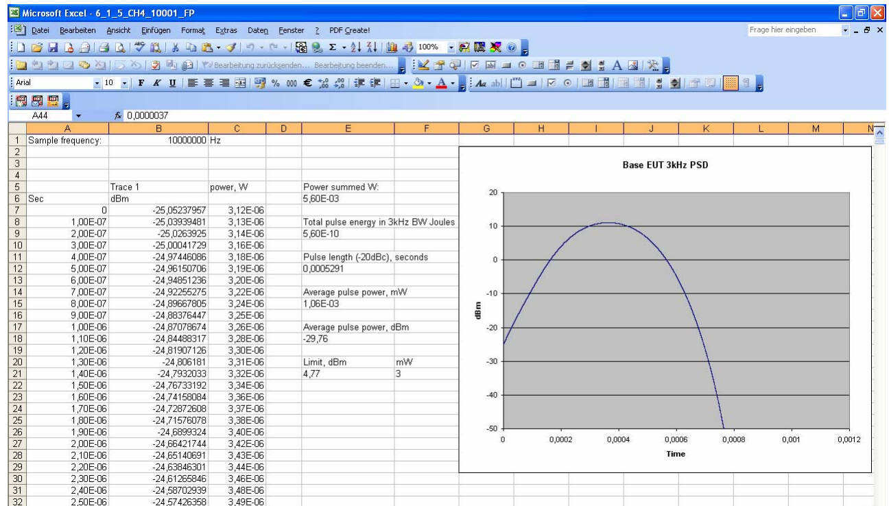
Screenshot of Excel file showing PSD calculations for base EUT, Lower Channel
