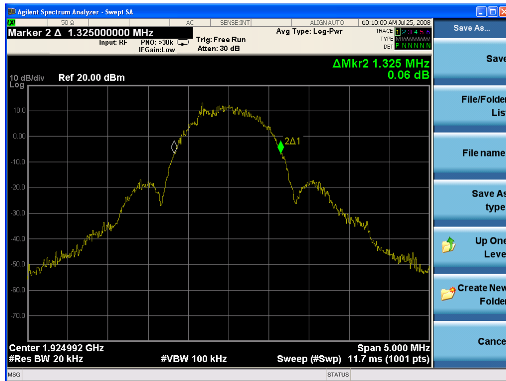
20 dB Bandwidth B, Middle Channel
