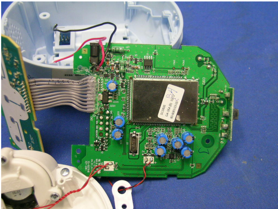
Baby Unit Main PCB comp side
