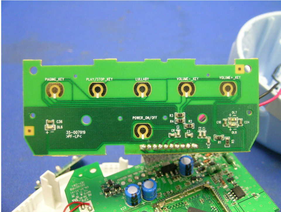
Baby Unit Keypad front side
