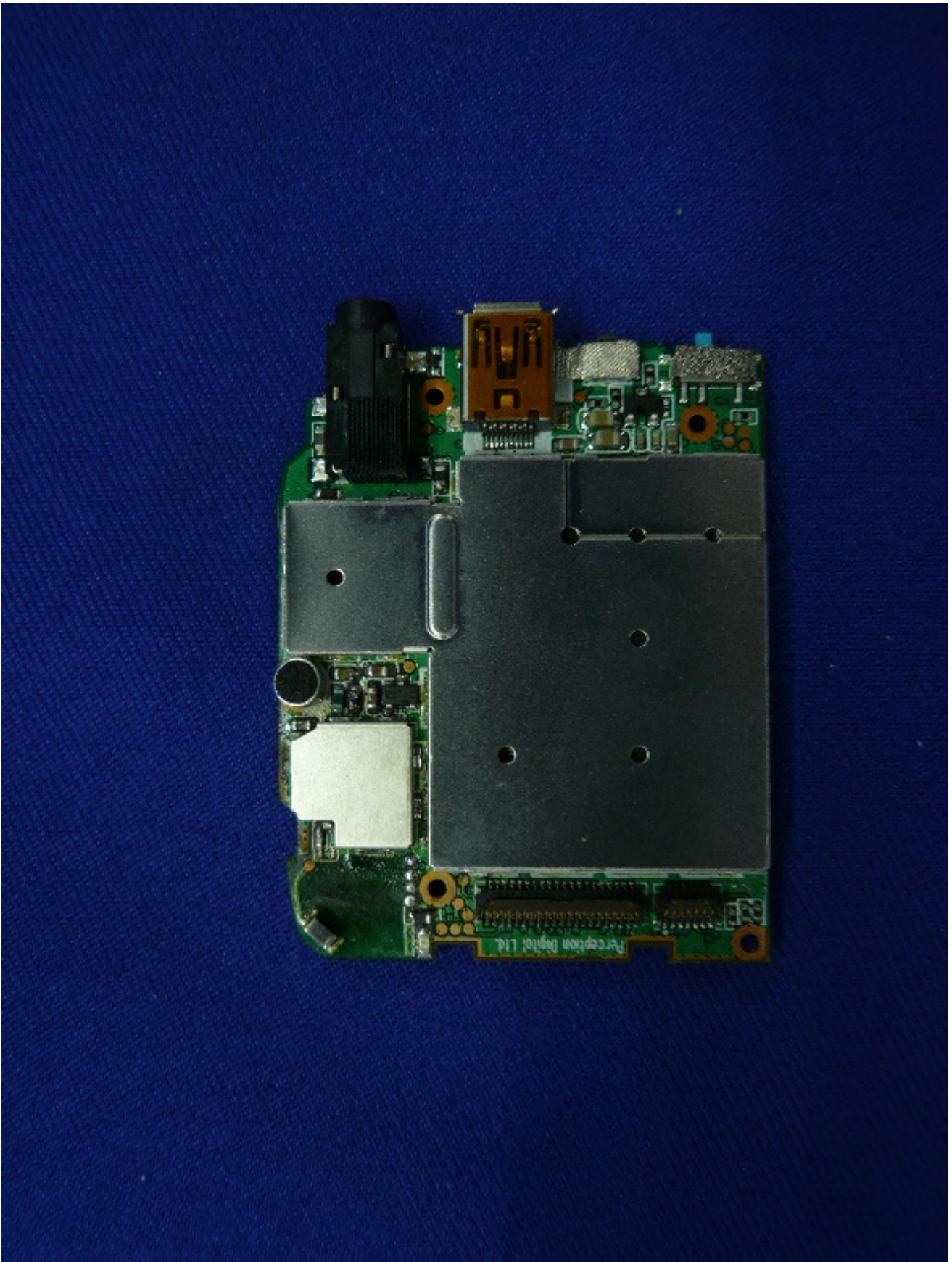
Figure 10 Inside of the EUT
