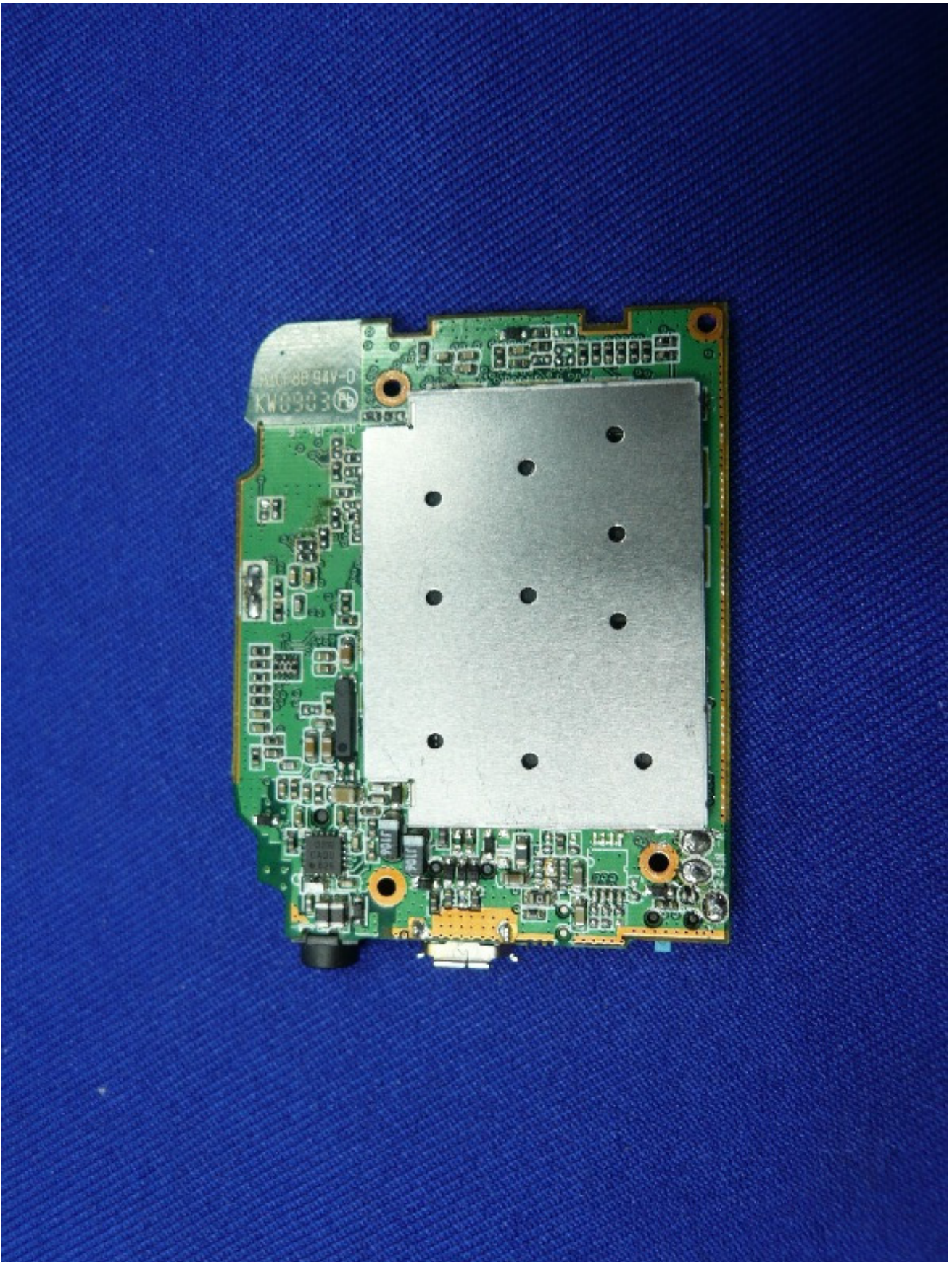
Figure 8 Inside of the EUT
