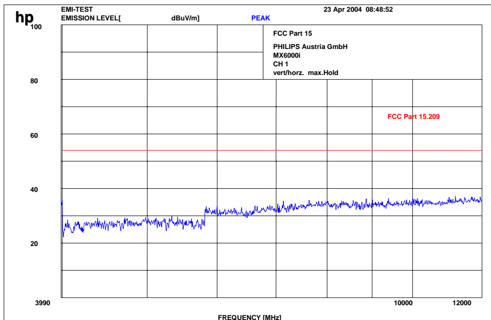
Plot 6: 4- 12 GHz vertical / horizontal (lowest channel)
