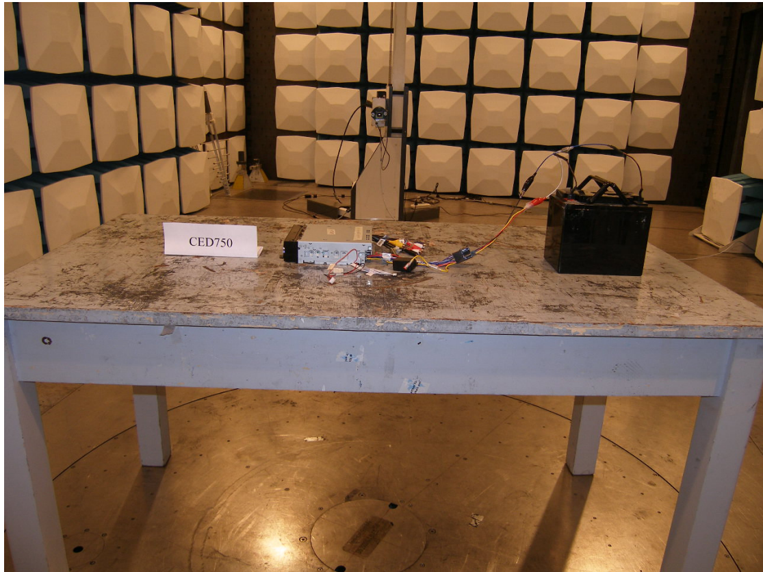
Photograph 3: Set-up for Radiation Measurement 18-25GHz
