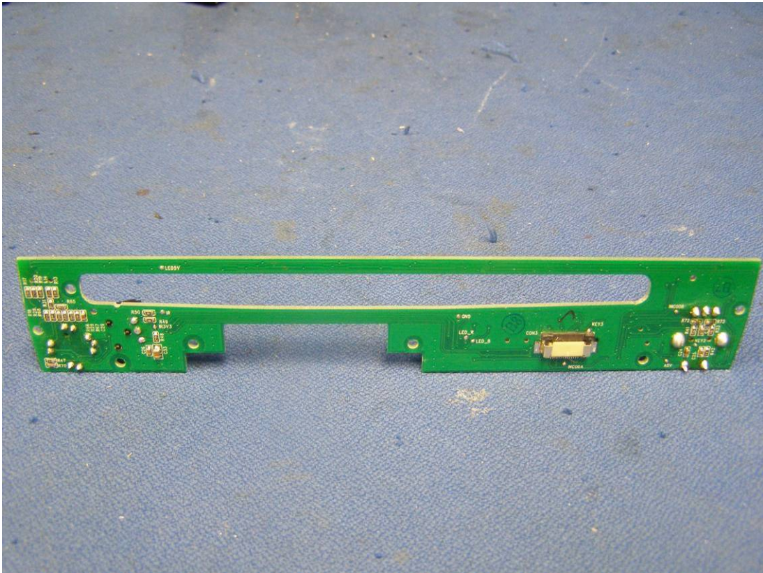
Picture 3(back side of main key board)
