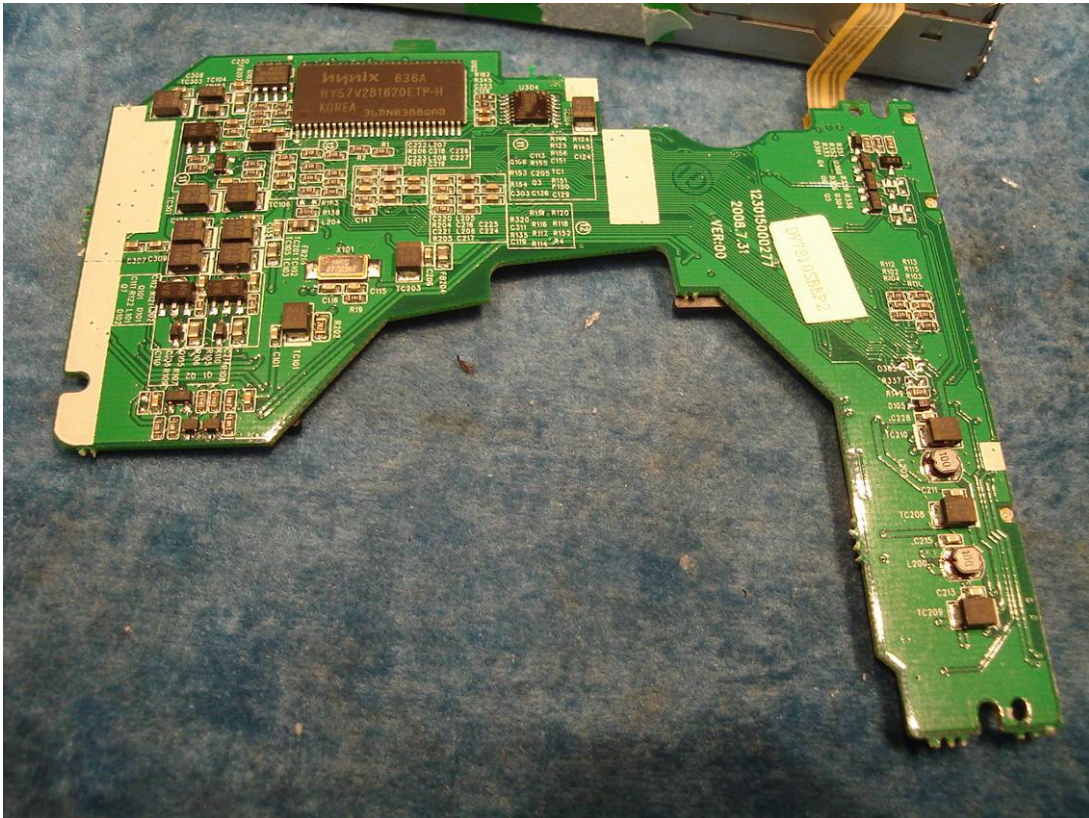
Picture 15 (back side of servo board)
