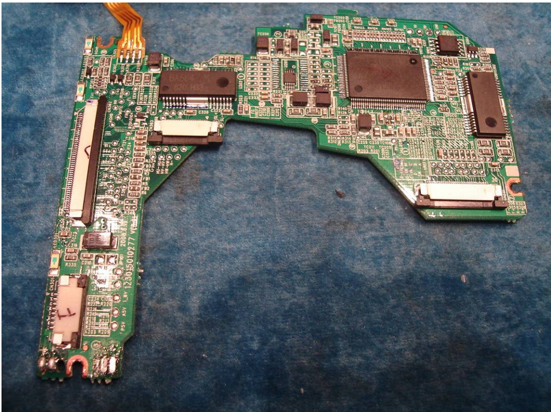
Picture 14 (front side of servo board)
