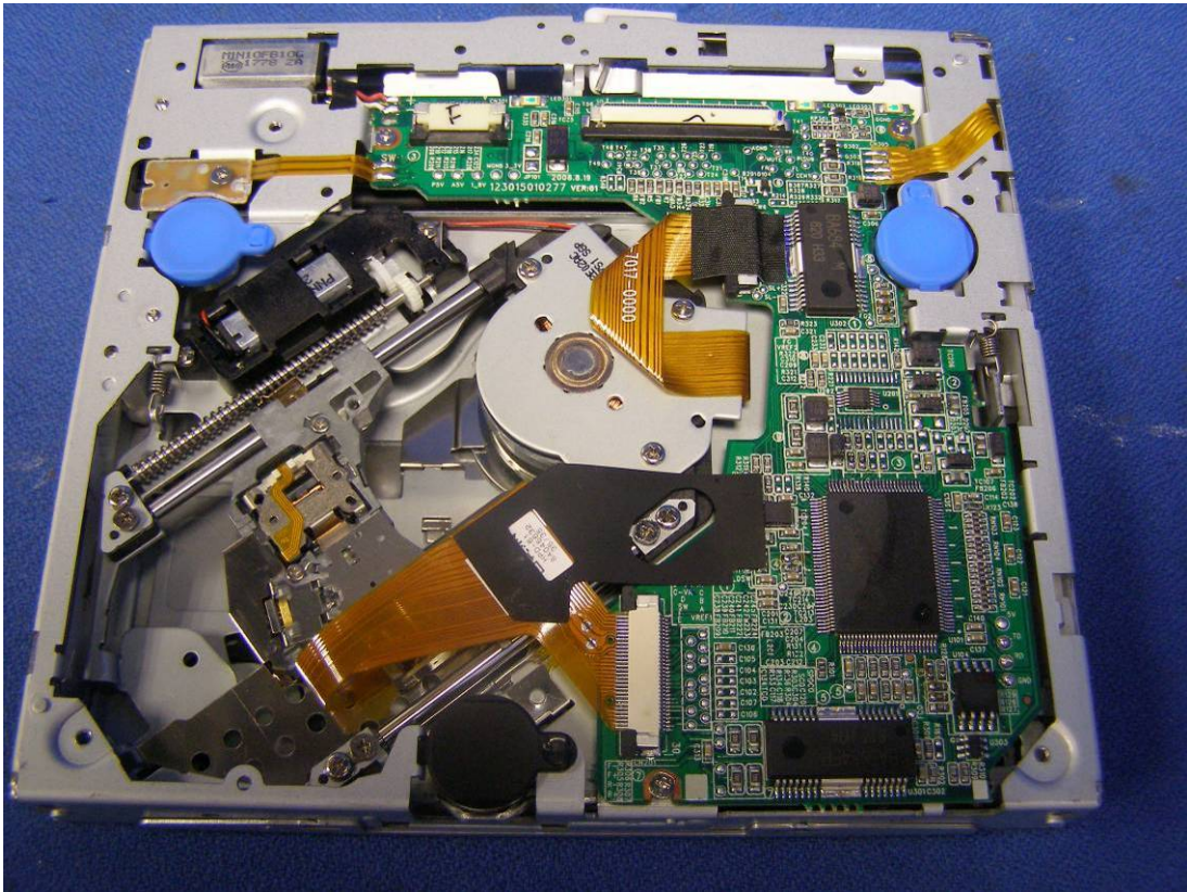
Picture 13 (DVD deck)
