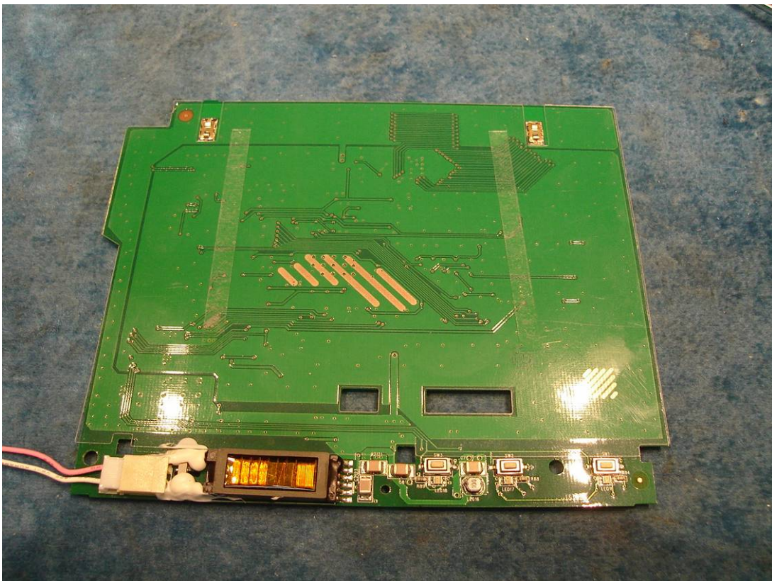
Picture 20 (back side of TFT driver board)
