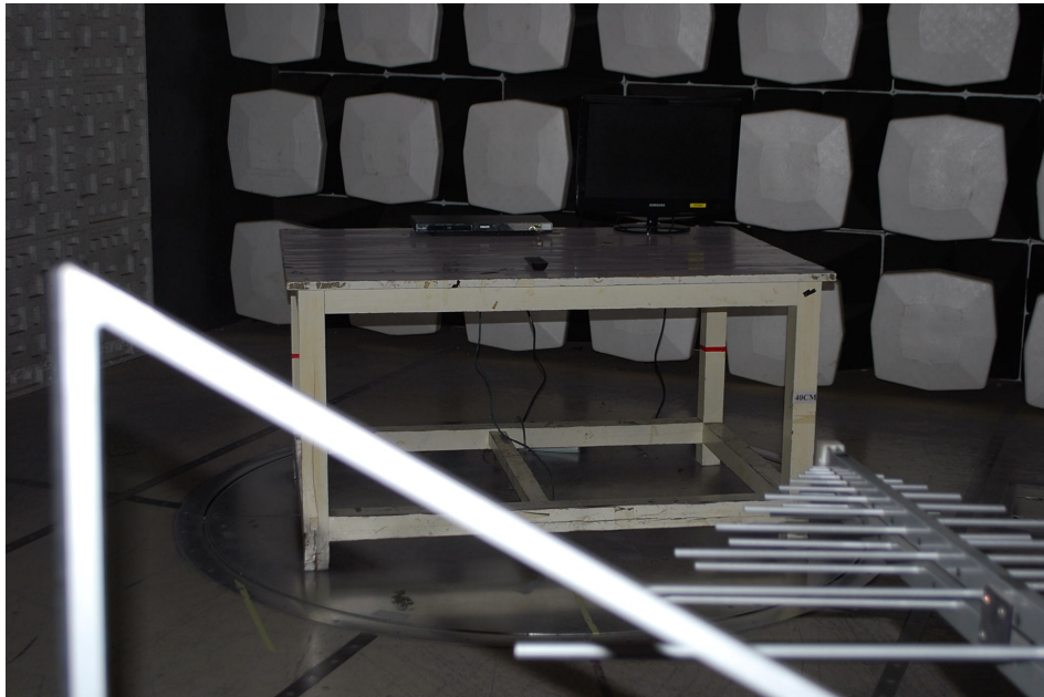
Radiated Emission
