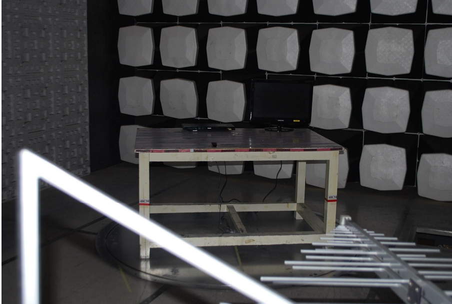
Radiated Emission
