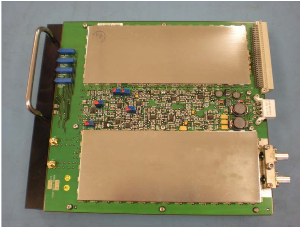
LOC PA with Shields
