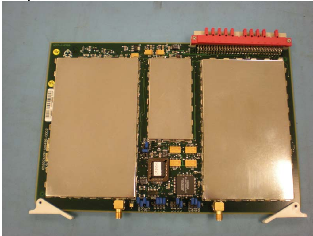
LOC Synthesizer with Shields
