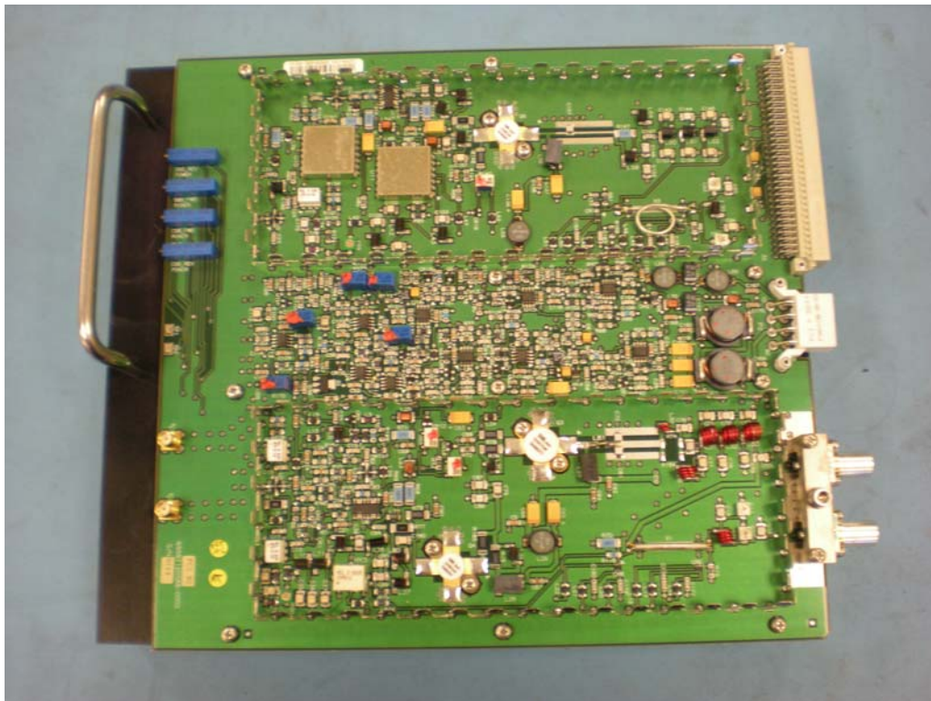
LOC PA without Shields
