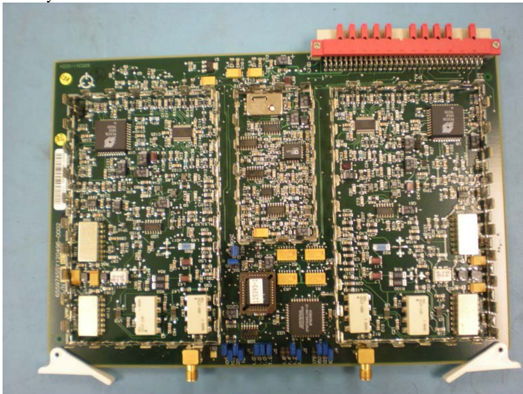
LOC Synthesizer without Shields
