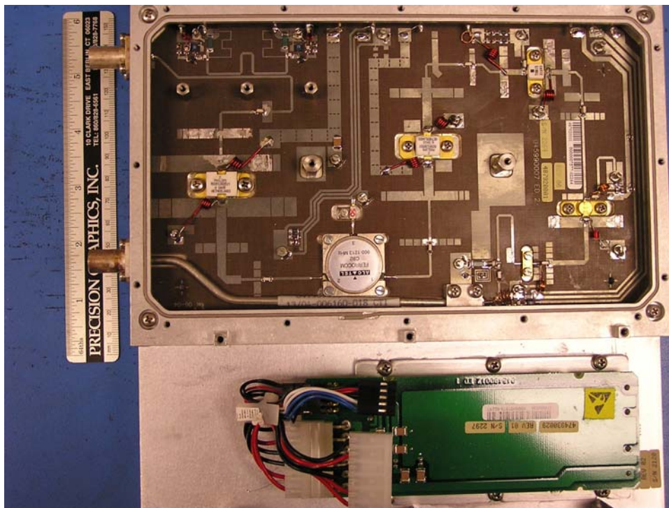
Transmitter amplifier chain
