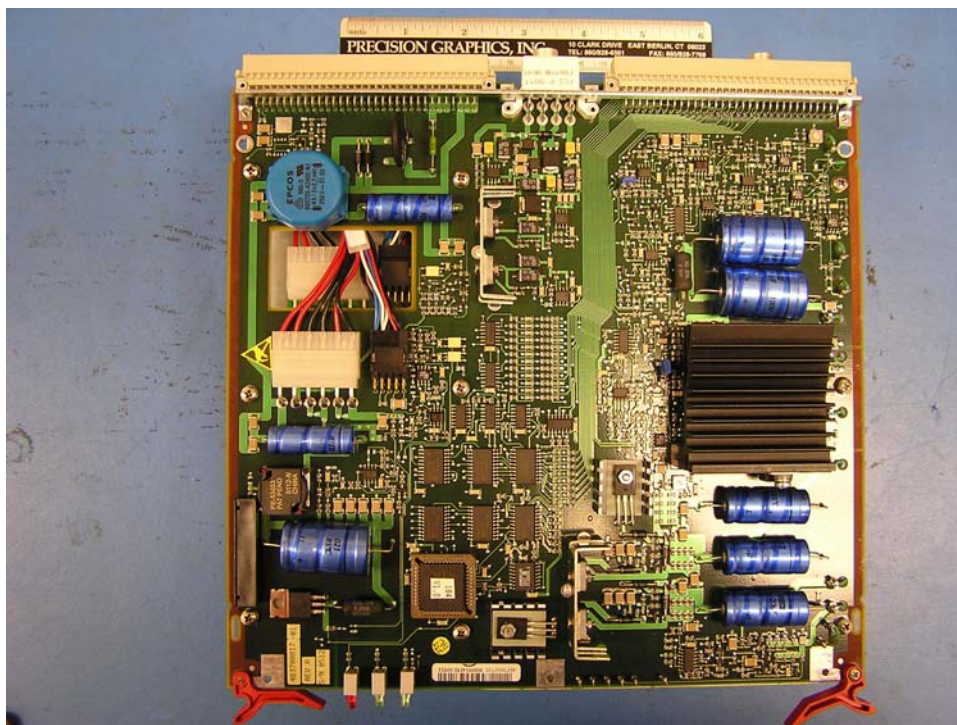
Assembled Transmitter
